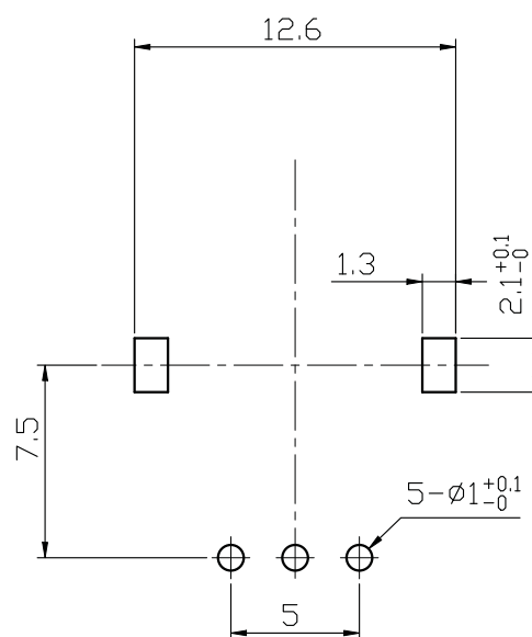
P. C. B. MOUNTING DETAIL
