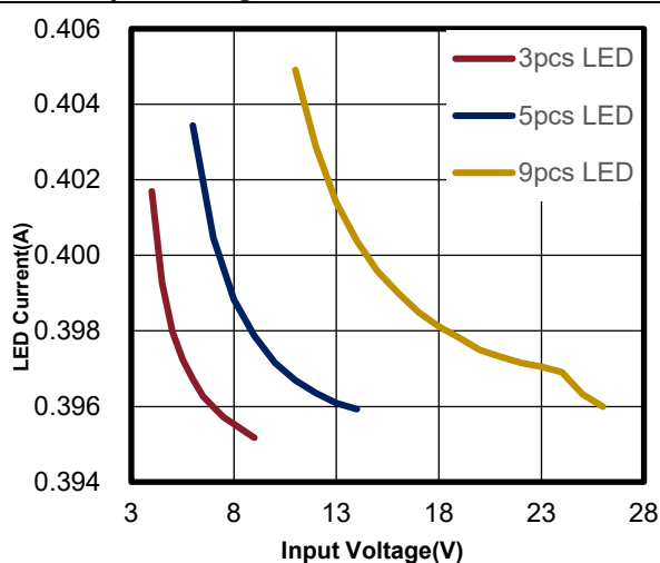
Figure 12.2.b I_{OUT}=400mA
