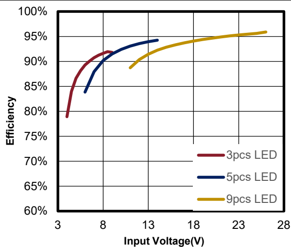
Figure 12.1.b I_{OUT}=400mA
