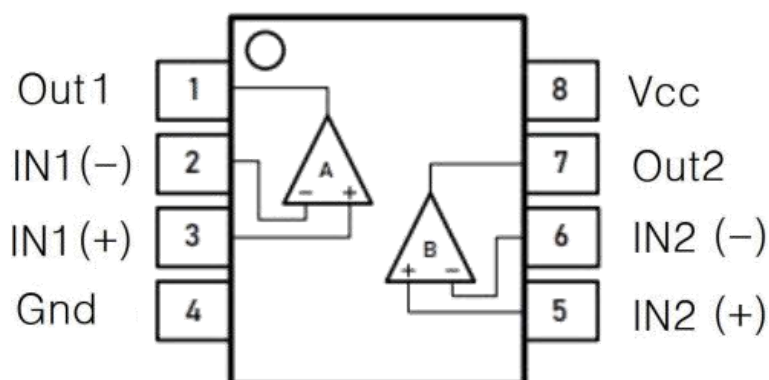
SOP-8
