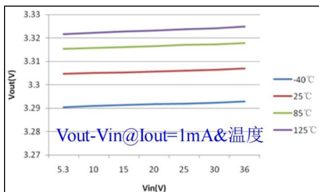
Line Regulation Iout=1mA
