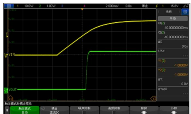
Vin=30V,Iout=30mA,Cout=10uF
