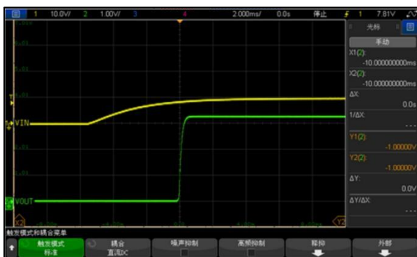
Vin=10V,Iout=30mA,Cout=0.1uF
