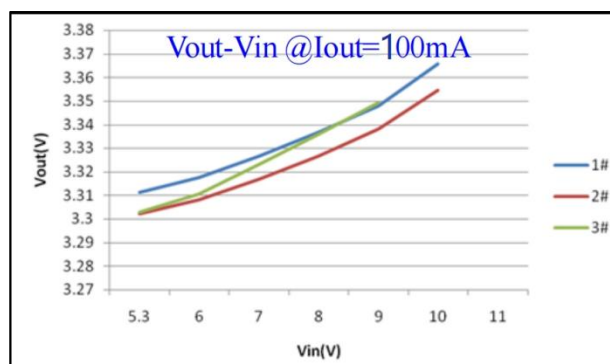
Iout=100mA Line Regulation
