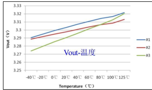
Output Voltage
