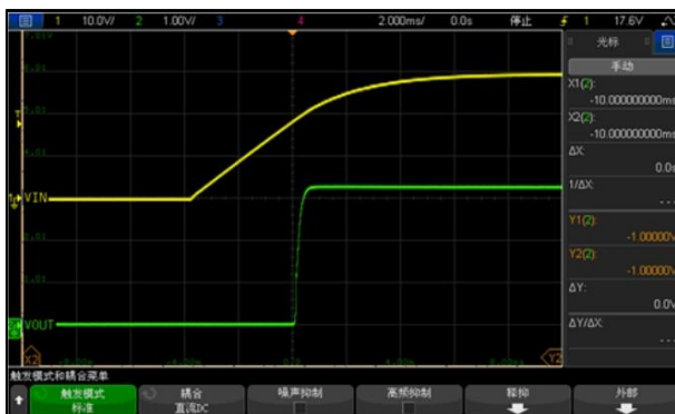
Vin=30V,Iout=30mA,Cout=0.1uF
