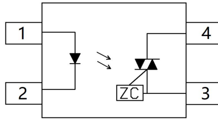
Pin Configuratic
