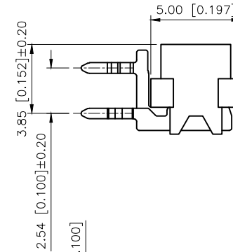
SECTION:A-A SCALE:1:1
