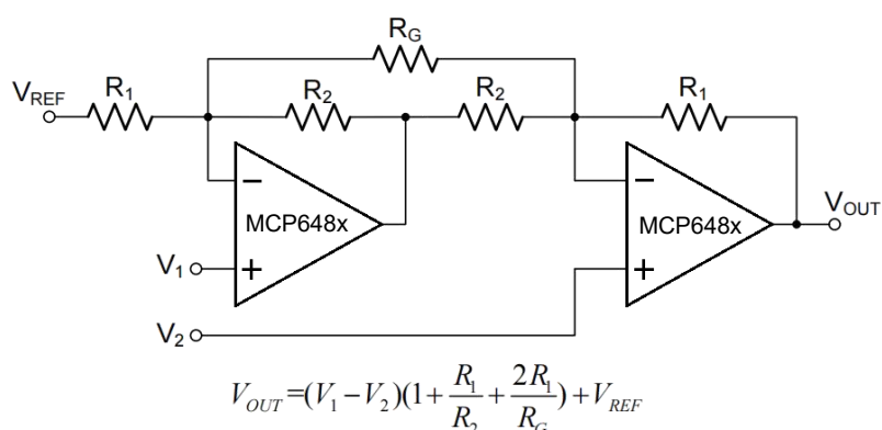
Figure 9. Instrumentation Amplifier
