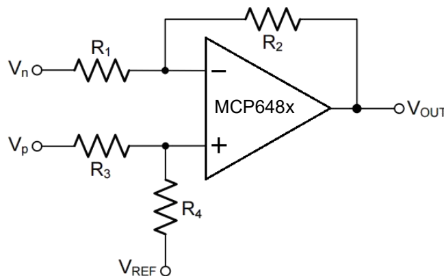
Figure 8. Differential Amplifier
