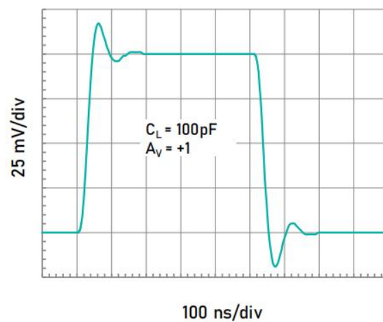
Small Signal Step Response (500 mV).
