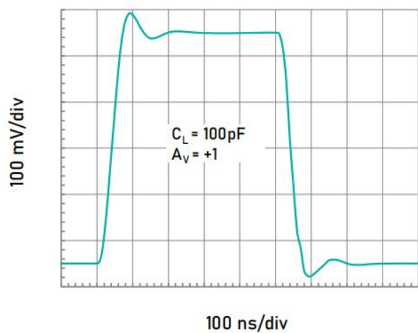
Small Signal Step Response (500 mV).
