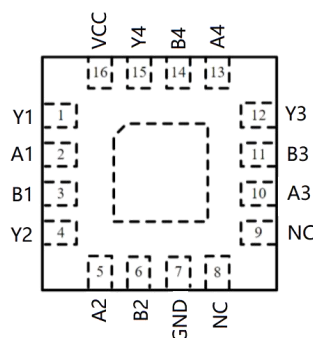
QFN-16 3*3
