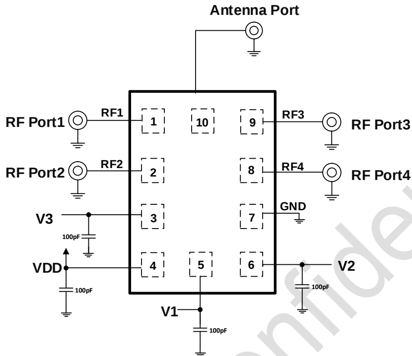
Figure 3. MXD8544B Application Circuit
