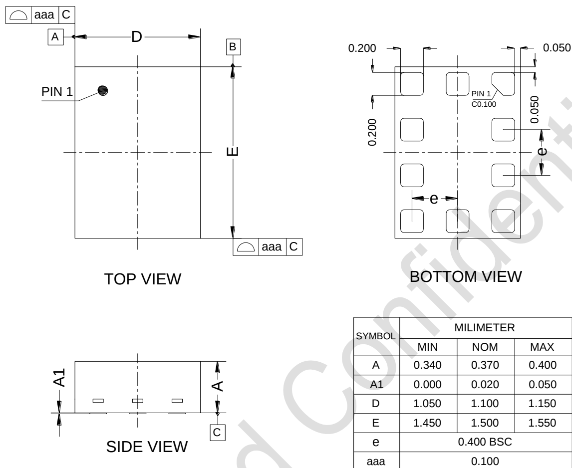
Figure 4. Package outline dimension
