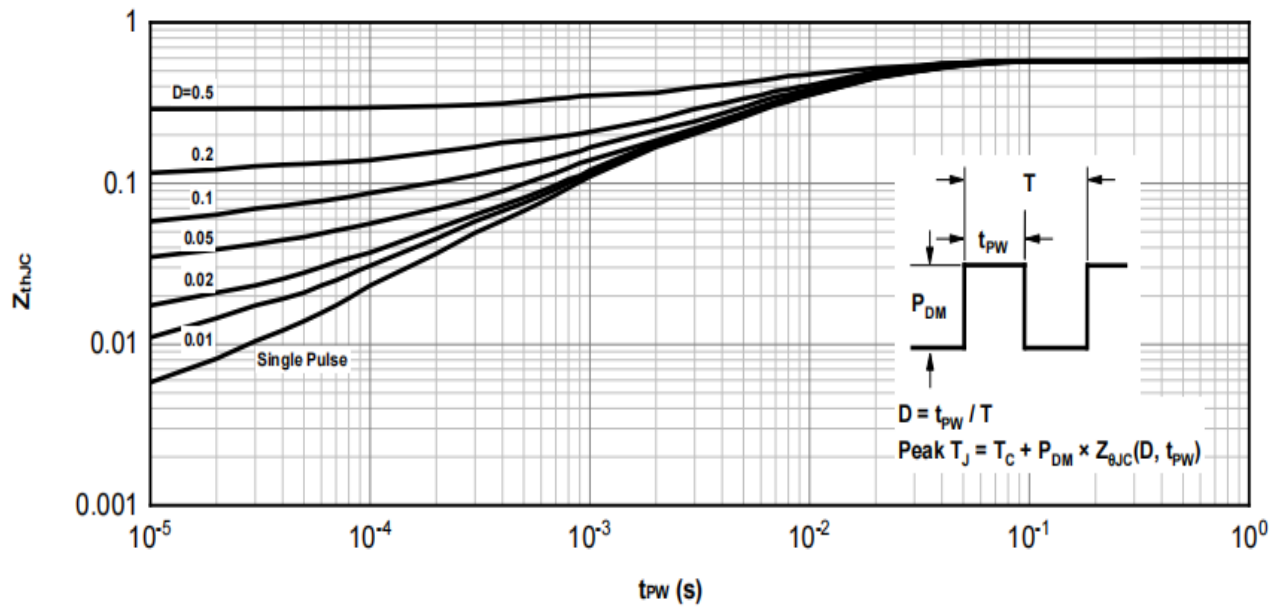
Fig.15 Transient thermal impedance from junction to case
