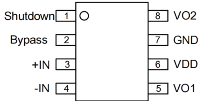
LM4871 Pin Diagram
