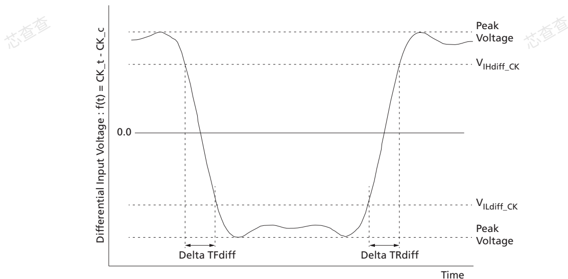
Figure 144: Differential Input Slew Rate Definition for CK t , CK c
