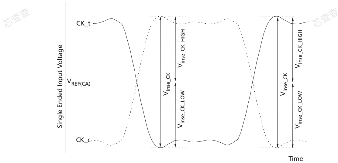
Figure 143: Clock Single-Ended Input Voltage
