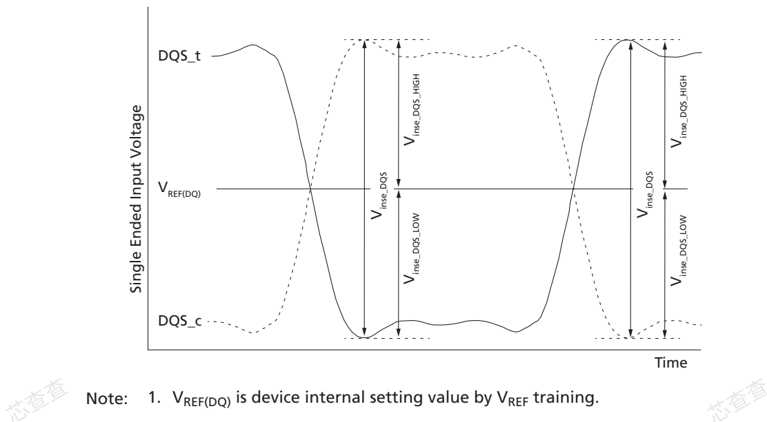
Figure 148: DQS Single-Ended Input Voltage
