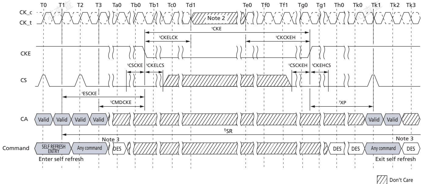
Figure 71: Command Input Timings after Power-Down Exit during Self Refresh
