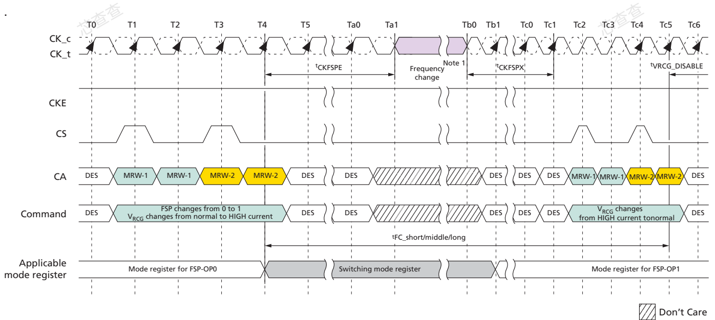
Figure 129: Frequency Set Point Switching Timing
