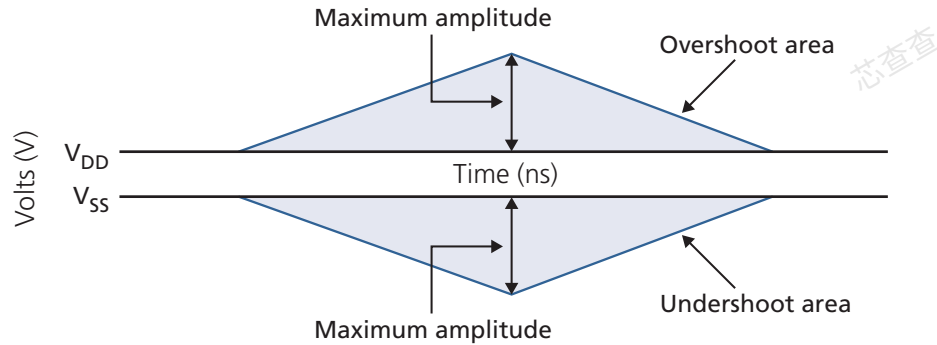
Figure 153: Overshoot and Undershoot Definition
