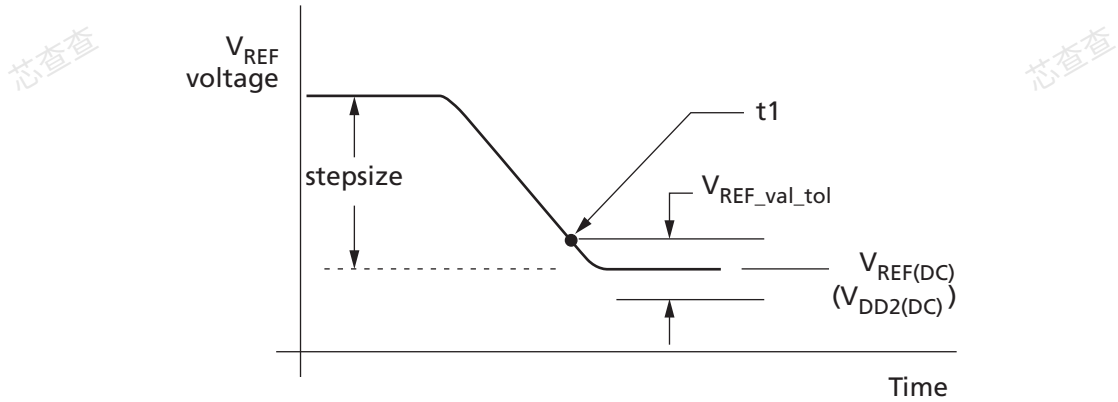
Figure 96: V REF(CA) Full Step from V REF,min to V REF,max
