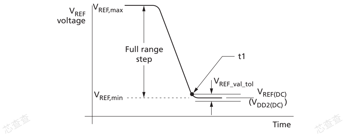
Figure 97: V REF(CA) Full Step from V REF,max to V REF,min
