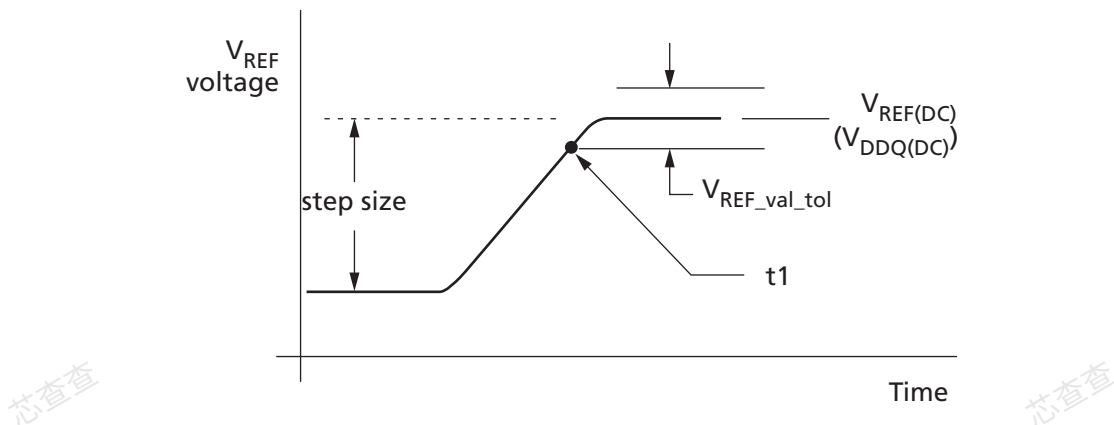
Figure 101: V REF(DQ) Single-Step Size Increment
