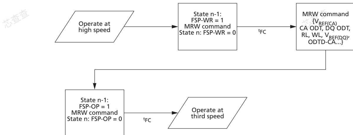
Figure 132: Example of Switching to a Third Trained Frequency Set Point
