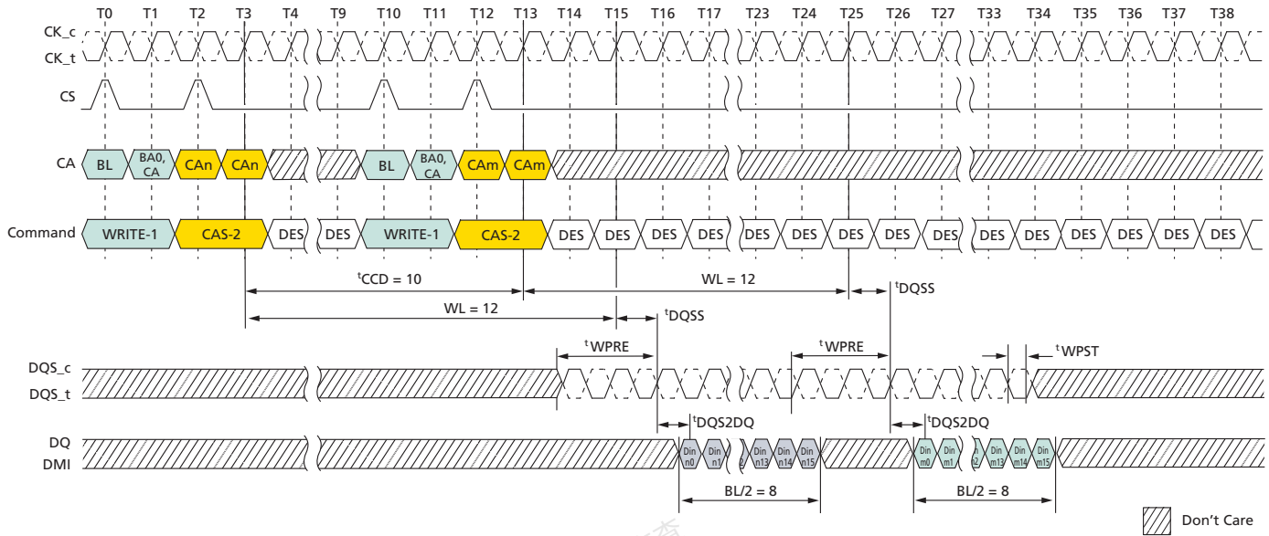
Figure 52: Consecutive Write: t_{CCD} = \text{Min} + 2, 0.5nCK Postamble
