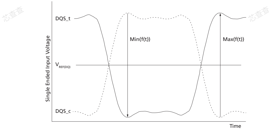
Figure 147: Definition of Differential DQS Peak Voltage
