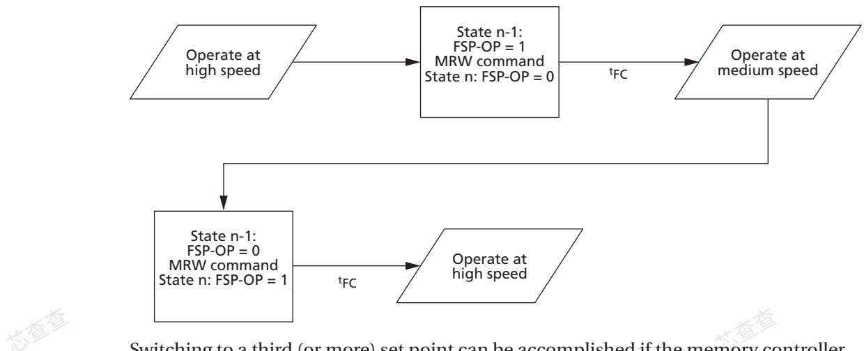
Figure 131: Example of Switching Between Two Trained Frequency Set Points
