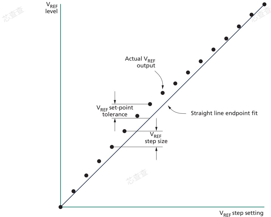
Figure 99: V_{REF} Set Tolerance and Step Size
