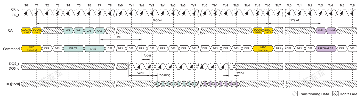
Figure 128: ZQCal Timing
