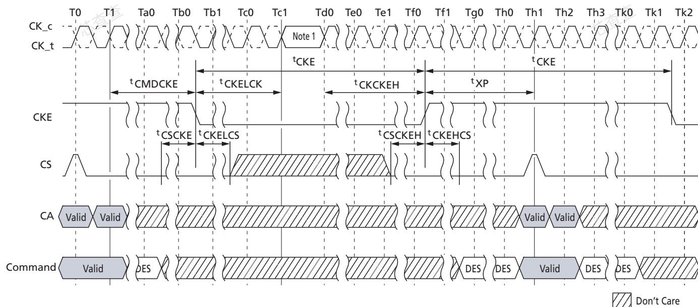
Figure 74: Basic Power-Down Entry and Exit Timing
