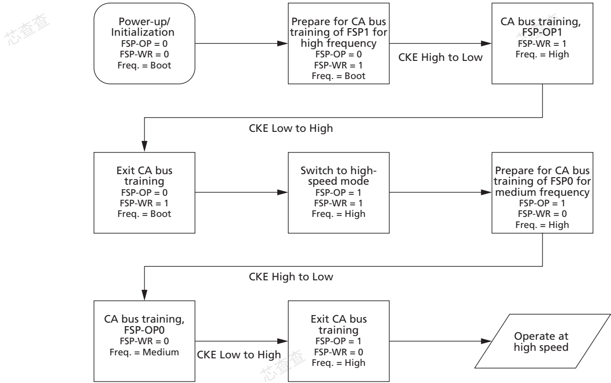
Figure 130: Training for Two Frequency Set Points
