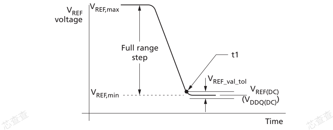
Figure 104: V REF(DQ) Full Step from V REF,max to V REF,min
