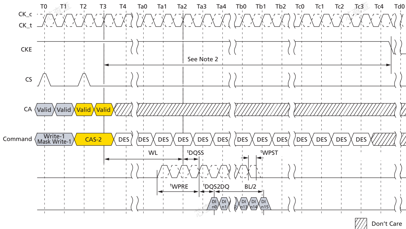
Figure 77: Write with Auto Precharge and Mask Write with Auto Precharge to Power-Down Entry
