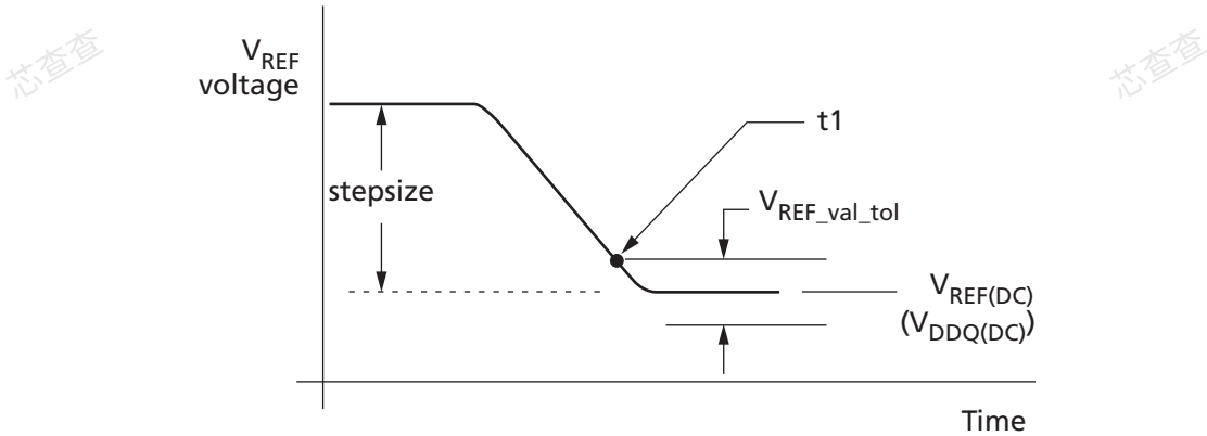
Figure 103: V REF(DQ) Full Step from V REF,min to V REF,max
