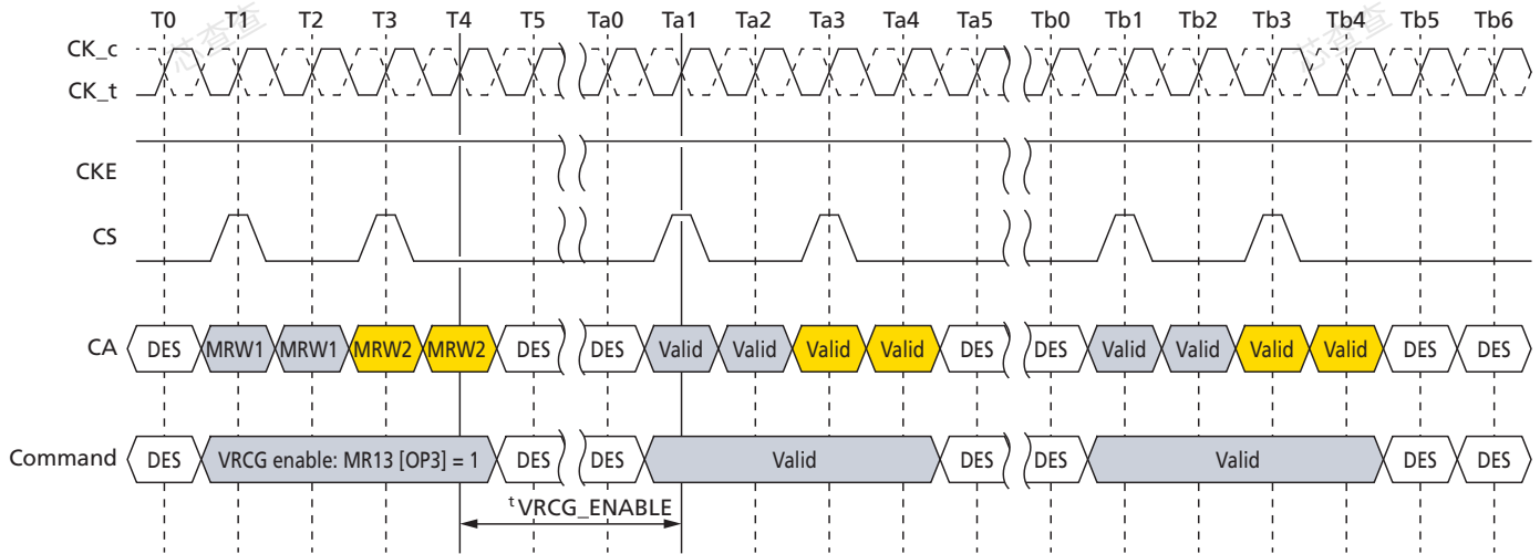
Figure 89: VRCG Enable Timing
