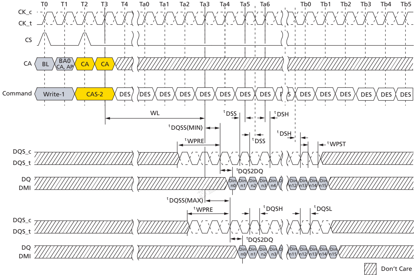
Figure 27: Write Timing
