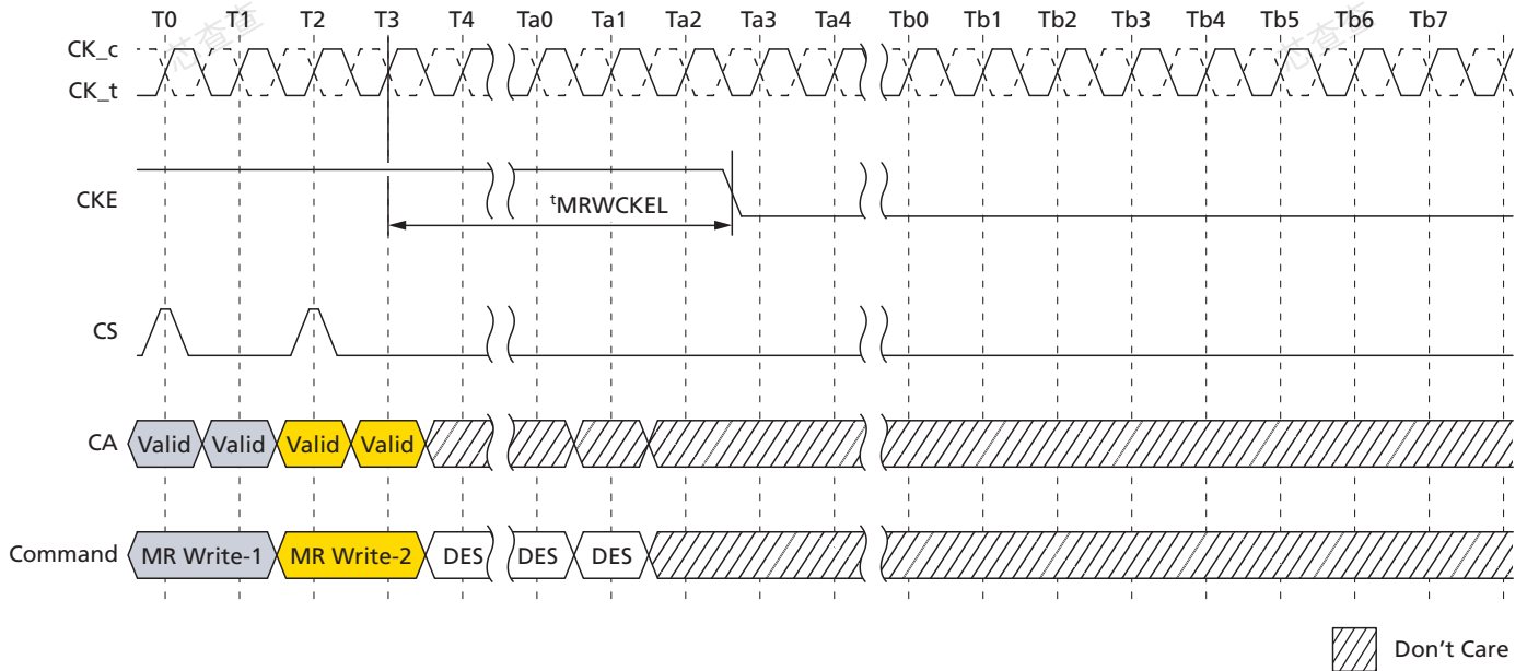
Figure 82: Mode Register Write to Power-Down Entry
