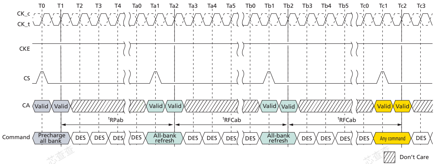
Figure 65: All-Bank REFRESH Operation
