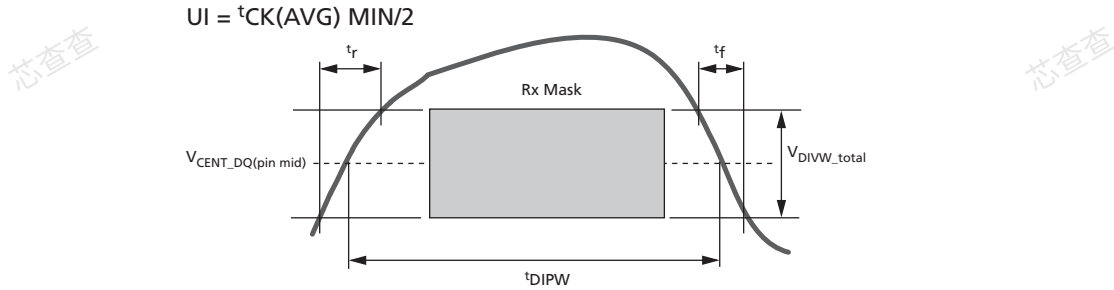
Figure 168: DQ t_{DIPW} and SRIN_divVW Definition for Each Input Pulse
