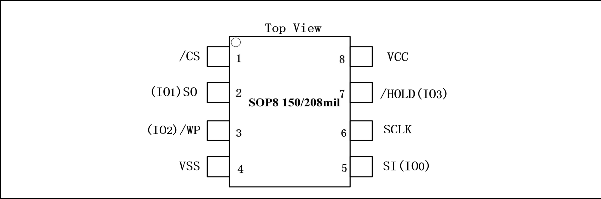
Figure 2. Pin Configuration SOP8 150/208 mil
