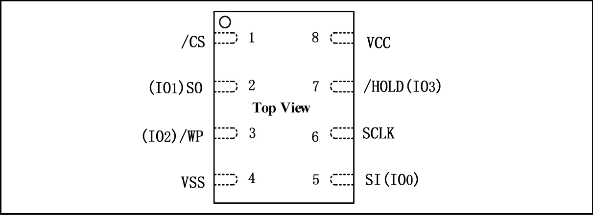
Figure 3. Pin Configuration USON8 2*3mm, USON8 4*3mm and WSON8 5*6mm
