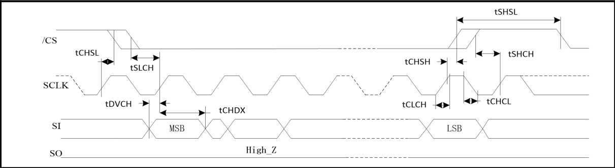
Figure 46. Output Timing
