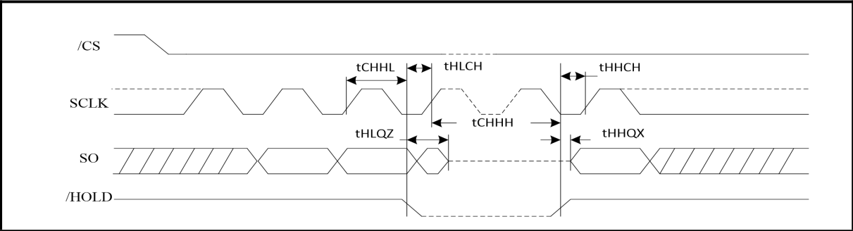
Figure 47. Hold Timing
