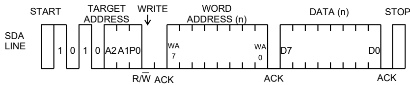
Figure 40. Byte Write
