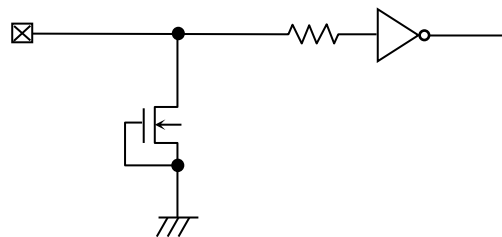
Figure 55. Input Pin Circuit Diagram (A1, A2, WP)
