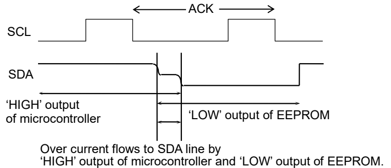
Figure 51. I/O Collision Timing
