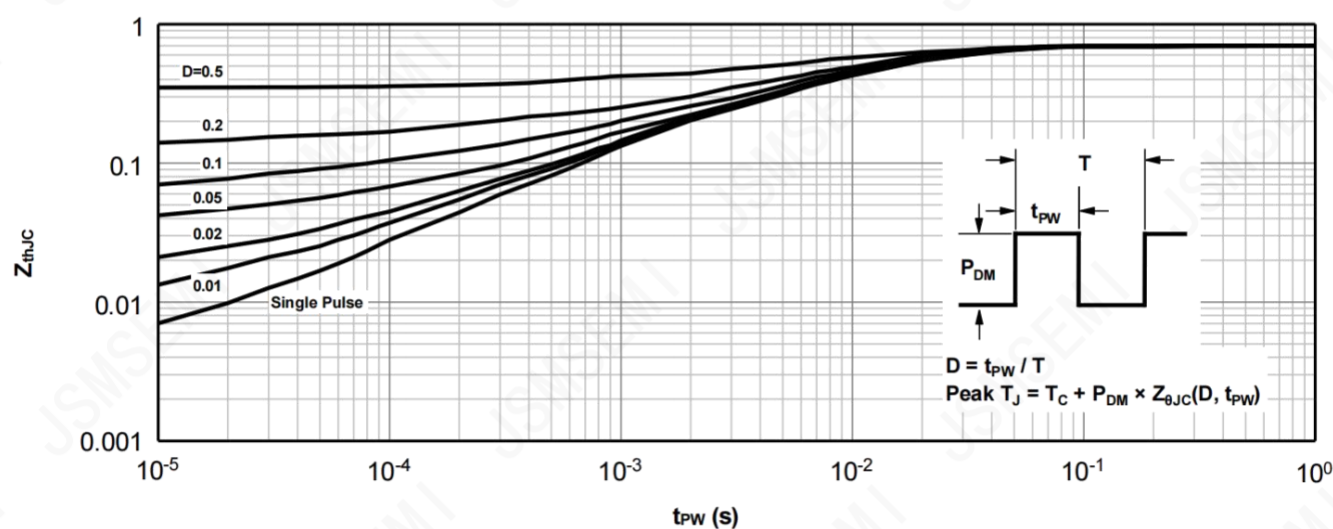
Figure 15: Normalized Transient Thermal Impedance Form Junction To Case
