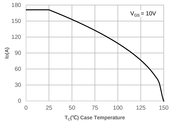
Figure 2: Current De-rating
