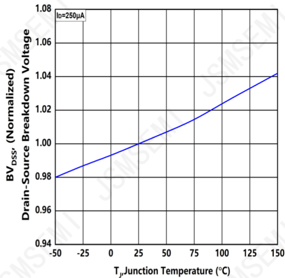
Figure.6 Typical Breakdown Voltage vs Junction Temperature
