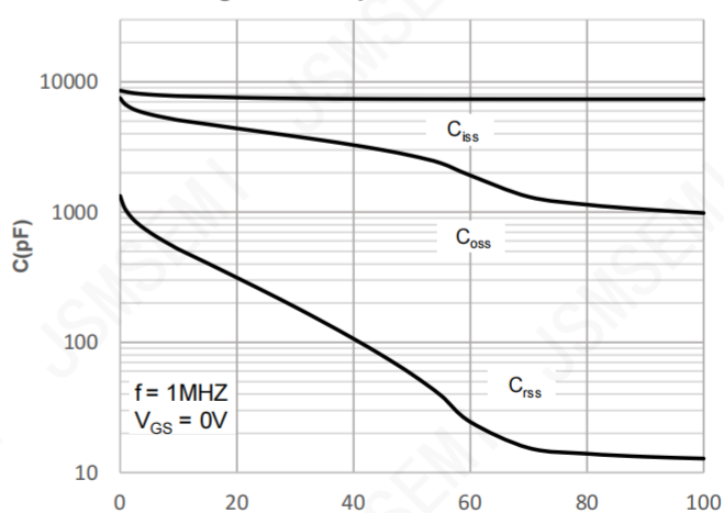
Figure 10: Capacitance Characteristics
