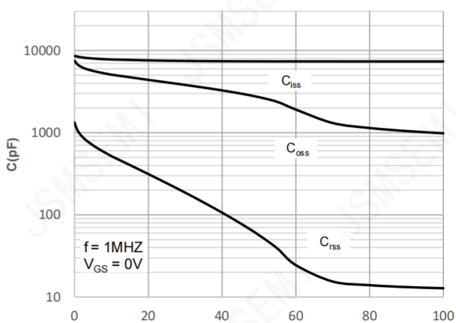
Figure 10: Capacitance Characteristics
