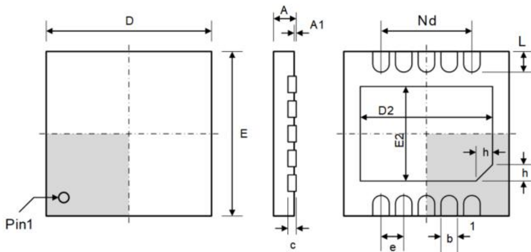
Figure 8. DFN10 package
