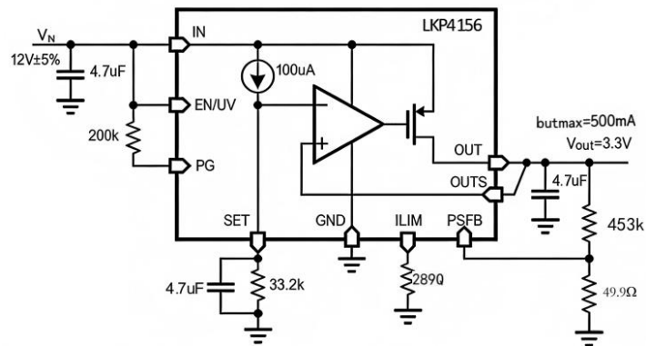
12Vin to 3.3Vout with 1.5VRMS Integrated Noise
