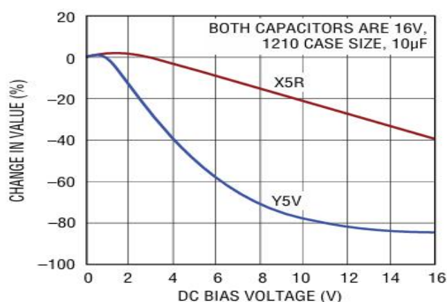
Figure 6. Ceramic Capacitor DC Bias Characteristics
