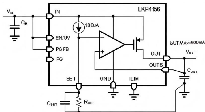
Figure 5. C_{OUT} and C_{SET} connections enhance stability
