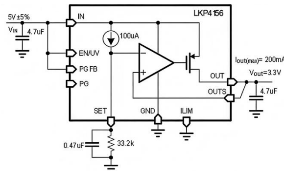
Figure 3. Typical adjustable voltage regulator
