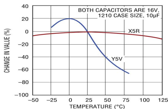
Figure 7. Ceramic Capacitor Temperature Characteristics
