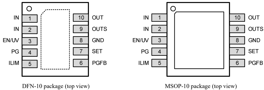
Figure 2. Pin Configuration
