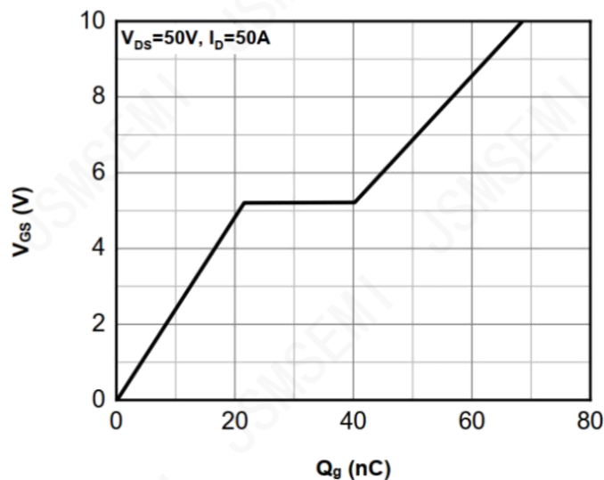
Figure 6: Typ. Gate Charge
