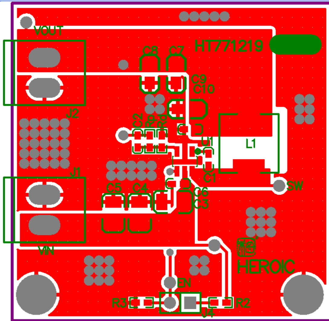
Figure 2 HT771219 Top Layer
