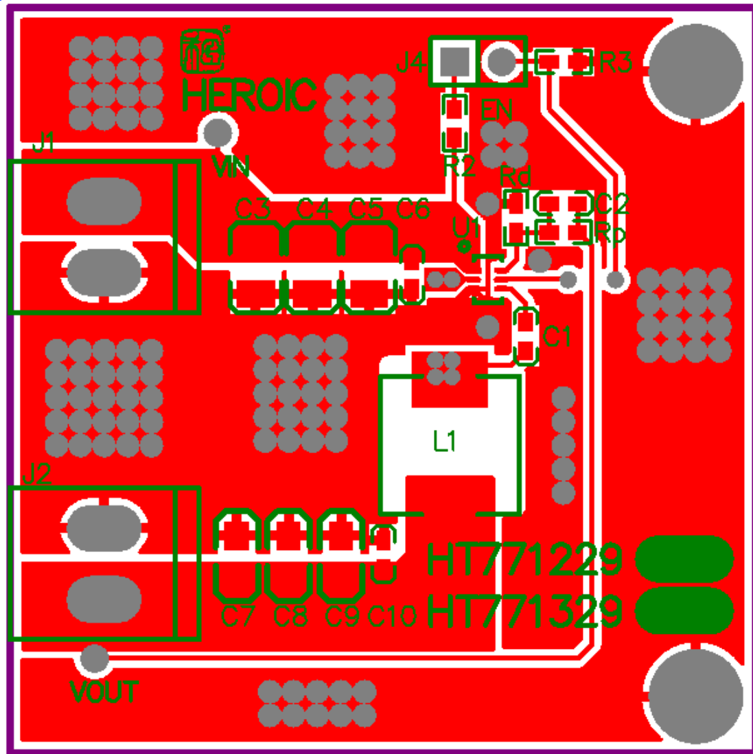
Figure 5 HT771229 Top Layer
