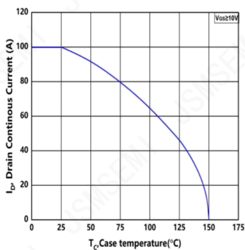
Figure.11 Continuous Drain Current Derating vs Case Temperature
