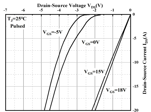
3rd Quadrant Characteristic at 25 °C
