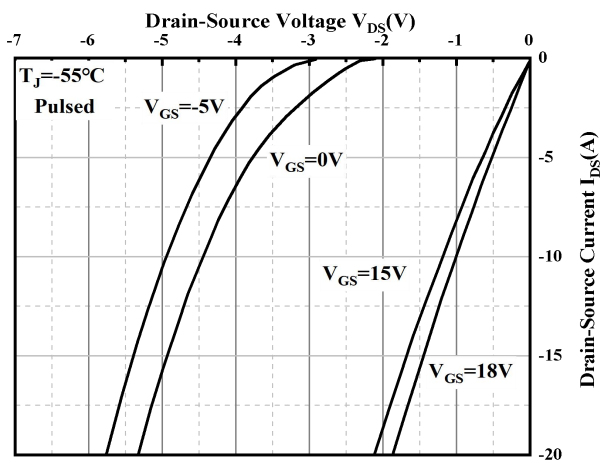
3rd Quadrant Characteristic at -55 °C
