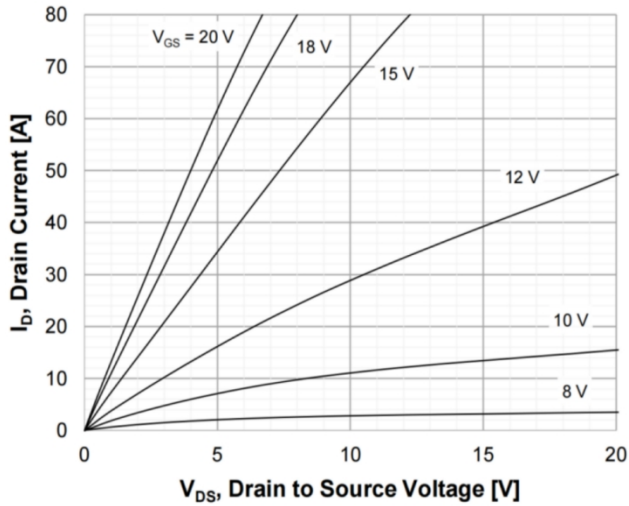
Figure 3. On-Region Characteristics T_J = 175^\circ\text{C}
