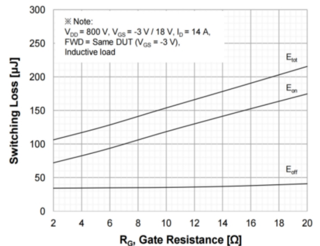
Figure 18. Typ. Switching Losses vs. Gate Resistance
