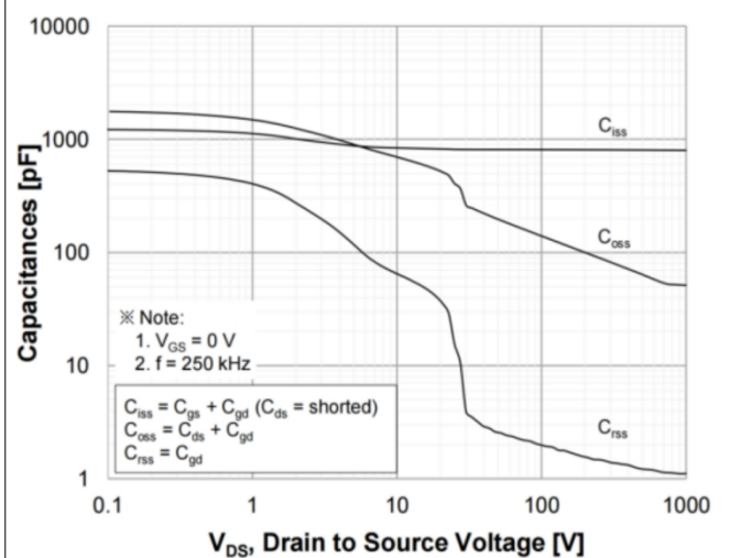
Figure 12. Capacitance Characteristics
