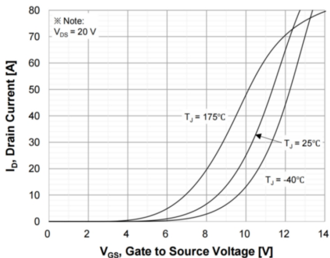
Figure 5. Transfer Characteristics
