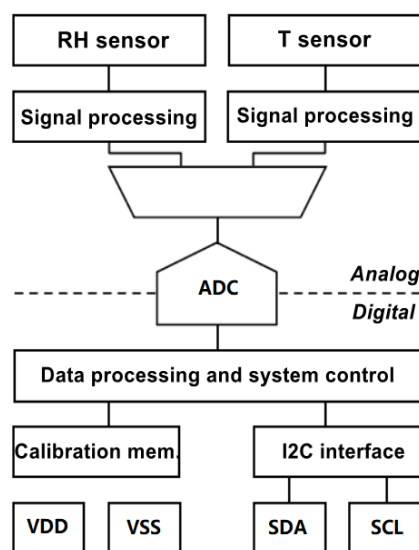
Figure 2. Functional block diagram of the SHTC3-P-NF
