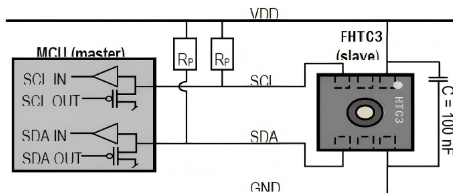
Figure 7. Typical application circuit for SHTC3-P-NF ( including pull-up resistors and decoupling capacitors)
