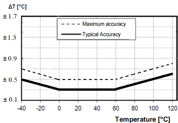
Figure 5. Temperature accuracy of SHTC3-P-NF
