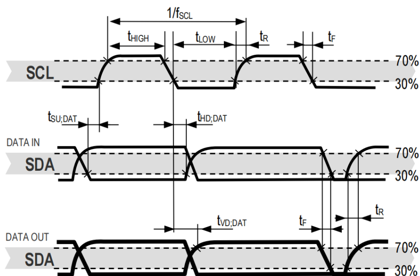
Figure 6. Timing diagram for digital input/output pads.
