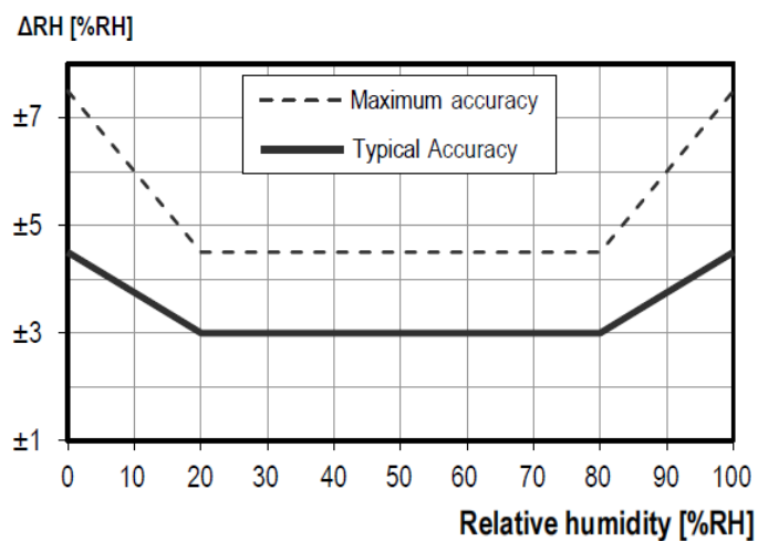
Figure 3. Tolerance of RH at 25 °C for SHTC3-P-NF
