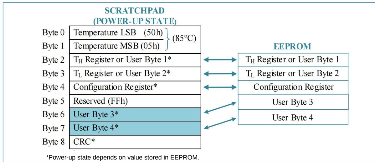
Figure 7. DS18B20-NF Memory Map
