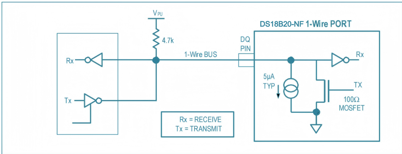
Figure 10. Hardware Configuration
