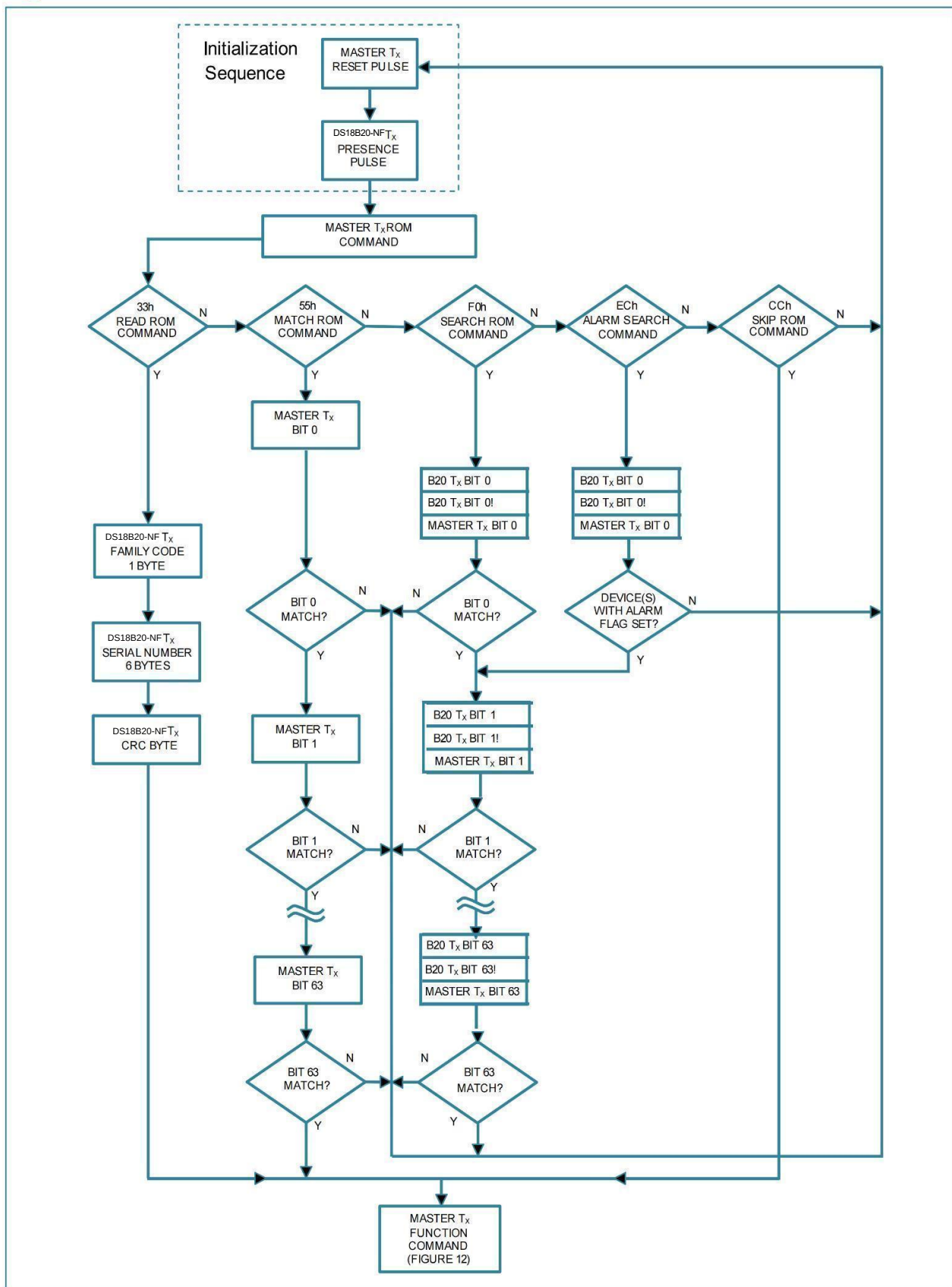
Figure 11. ROM Instruction Flowchart
