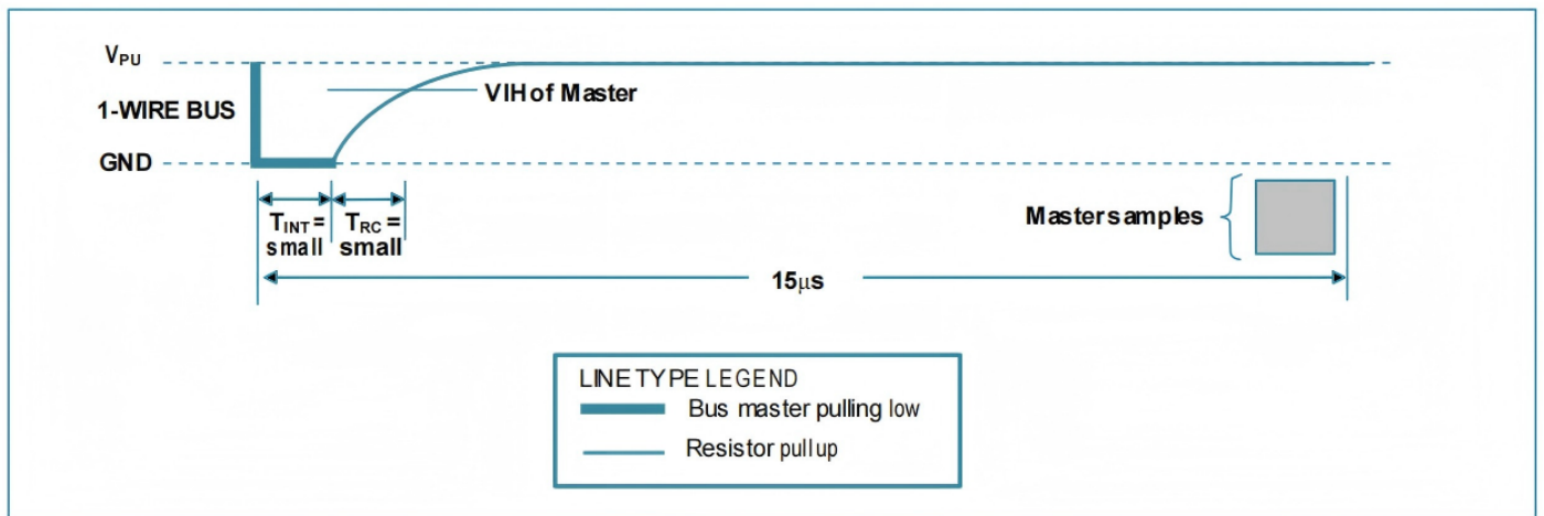
Figure 16. Recommended Master Read 1 Timing
