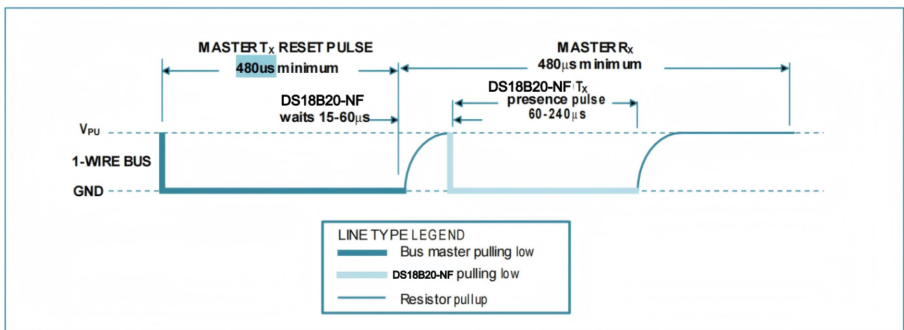
Figure 13. Initialization Timing
