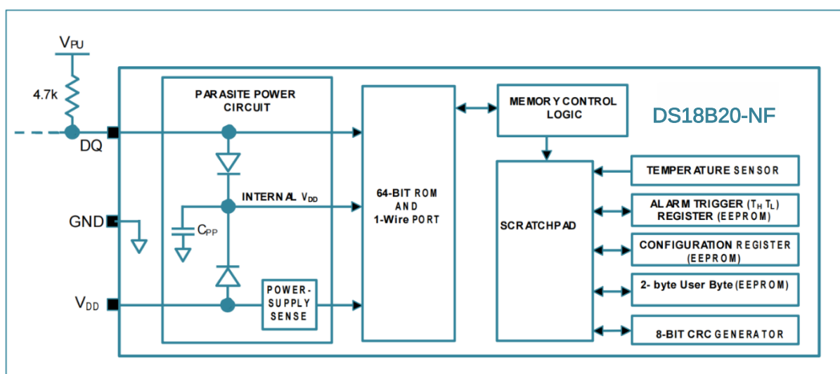
Figure 1. DS18B20-NF Block Diagram
