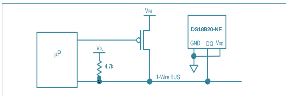
Figure 4. Supplying the Parasite-Powered DS18B20-NF During Temperature Conversions
