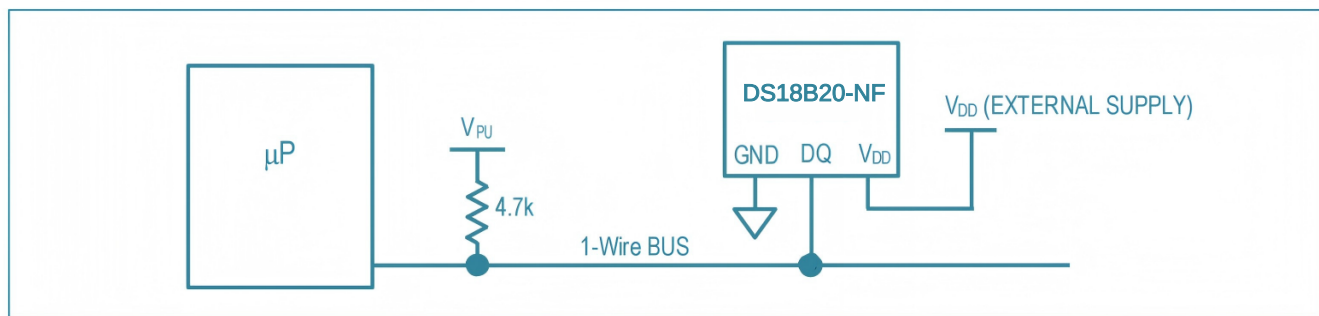
Figure 5. Powering the DS18B20-NF with an External Supply
