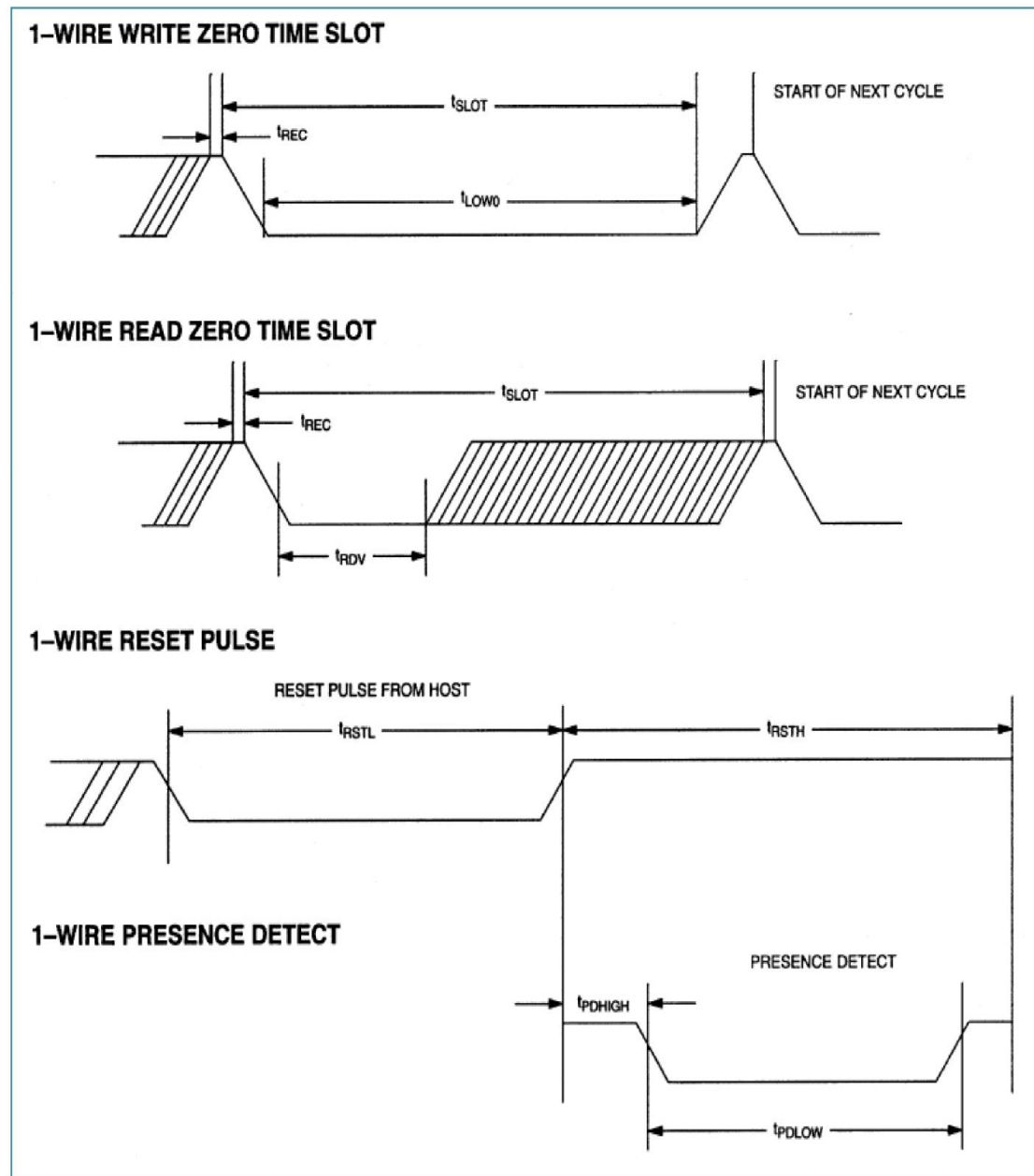
Figure 18. Timing Diagrams
