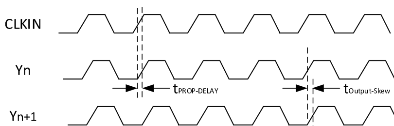
Propagation Delay t_{PROP-DELAY} and Output Skew t_{Output-SKEW}
