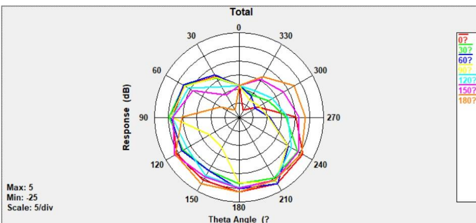
Total @2500 MHz
