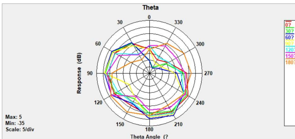
Theta @2500 MHz
