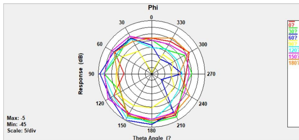
Phi @920 MHz
