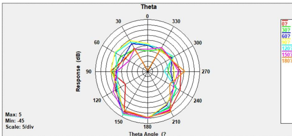
Theta @920 MHz
