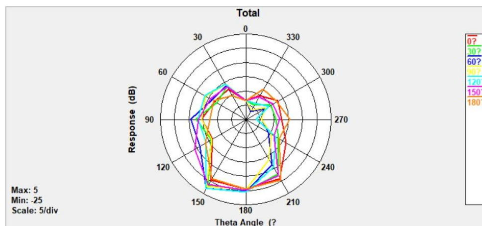
Total @920 MHz
