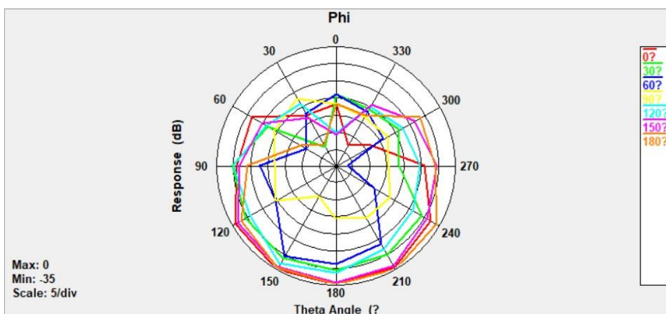
Phi @2500 MHz
