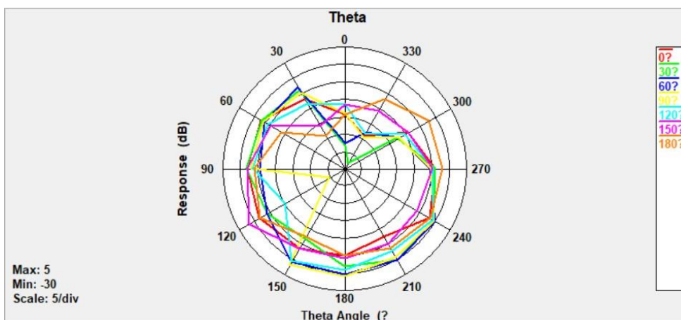
Theta @1800 MHz
