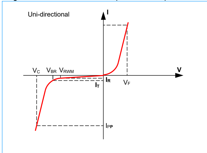
Fig1. V-I Curve Characteristics (Ui-directional)
