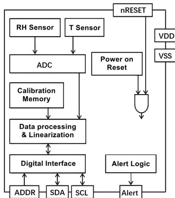
Figure 2. Functional block diagram of FHT30
