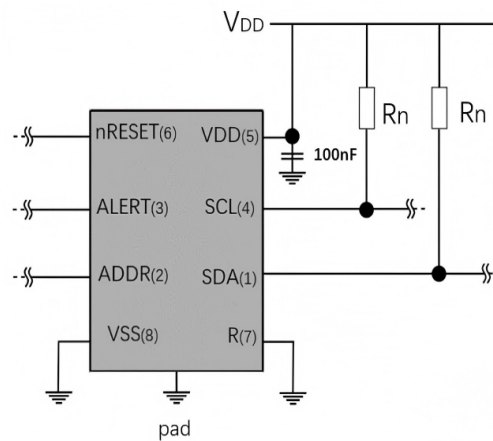
Figure 5. Typical Application Circuit.
