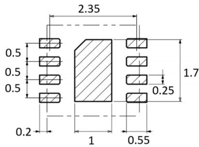
Figure 8. Recommended metal land pattern and stencil apertures for the FHT30.
