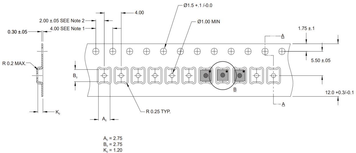
Figure 9. Dimensions of tape for chip transport.
