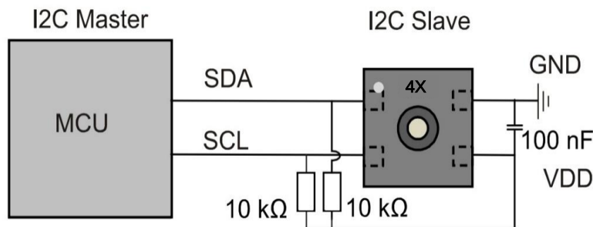
Figure 6 Typical application circuit reference diagram of FHT40
