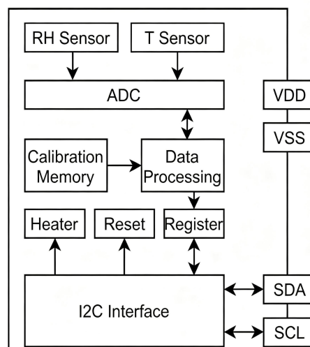
Functional Block Diagram of FHT40 Family
