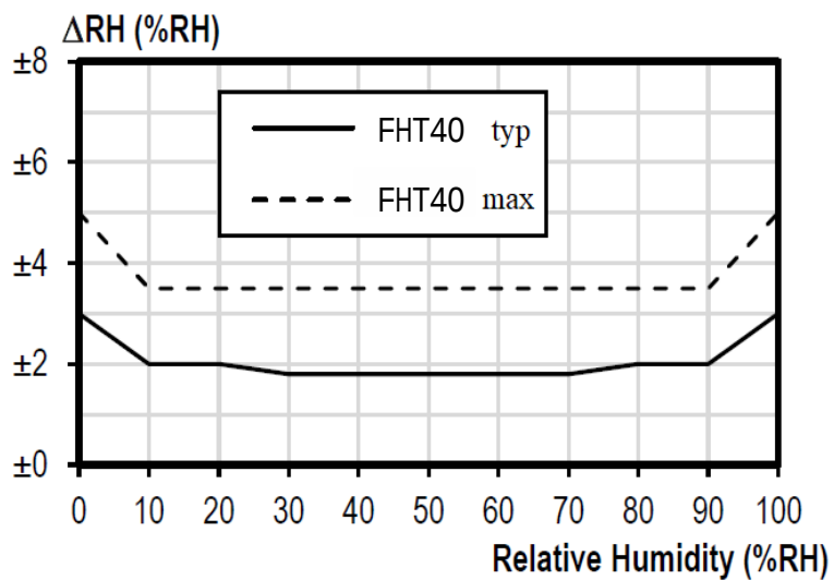
Figure 2 FHT40 RH accuracy @25°C
