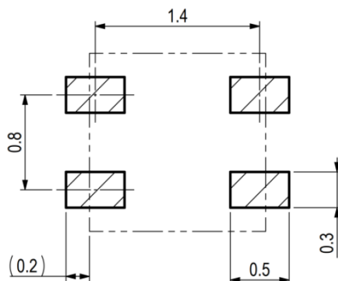
Figure 8 Recommended land pattern (in mm)
