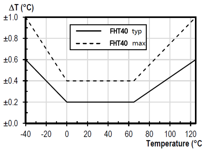
Figure 4 FHT40 temperature accuracy
