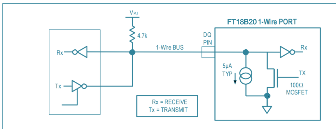
Figure 10. Hardware Configuration
