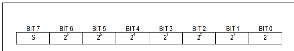
Figure 3. TH and TL Register Format
