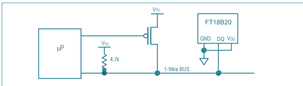
Figure 4. Supplying the Parasite-Powered FT18B20 During Temperature Conversions
