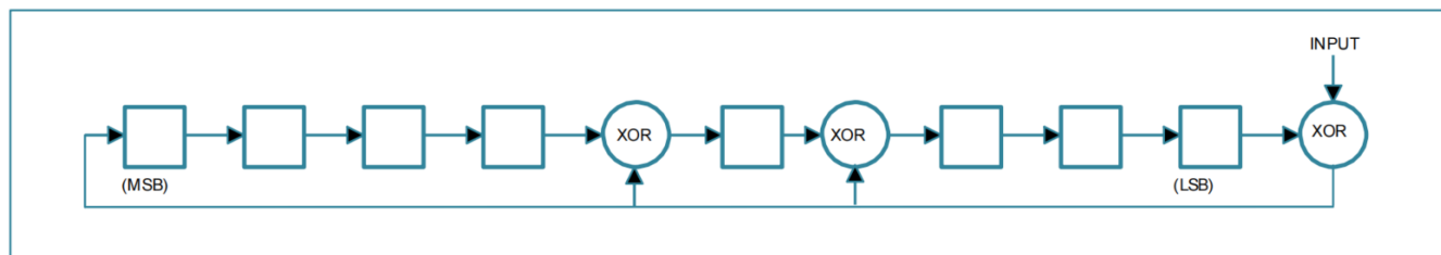
Figure 9. CRC Generator
