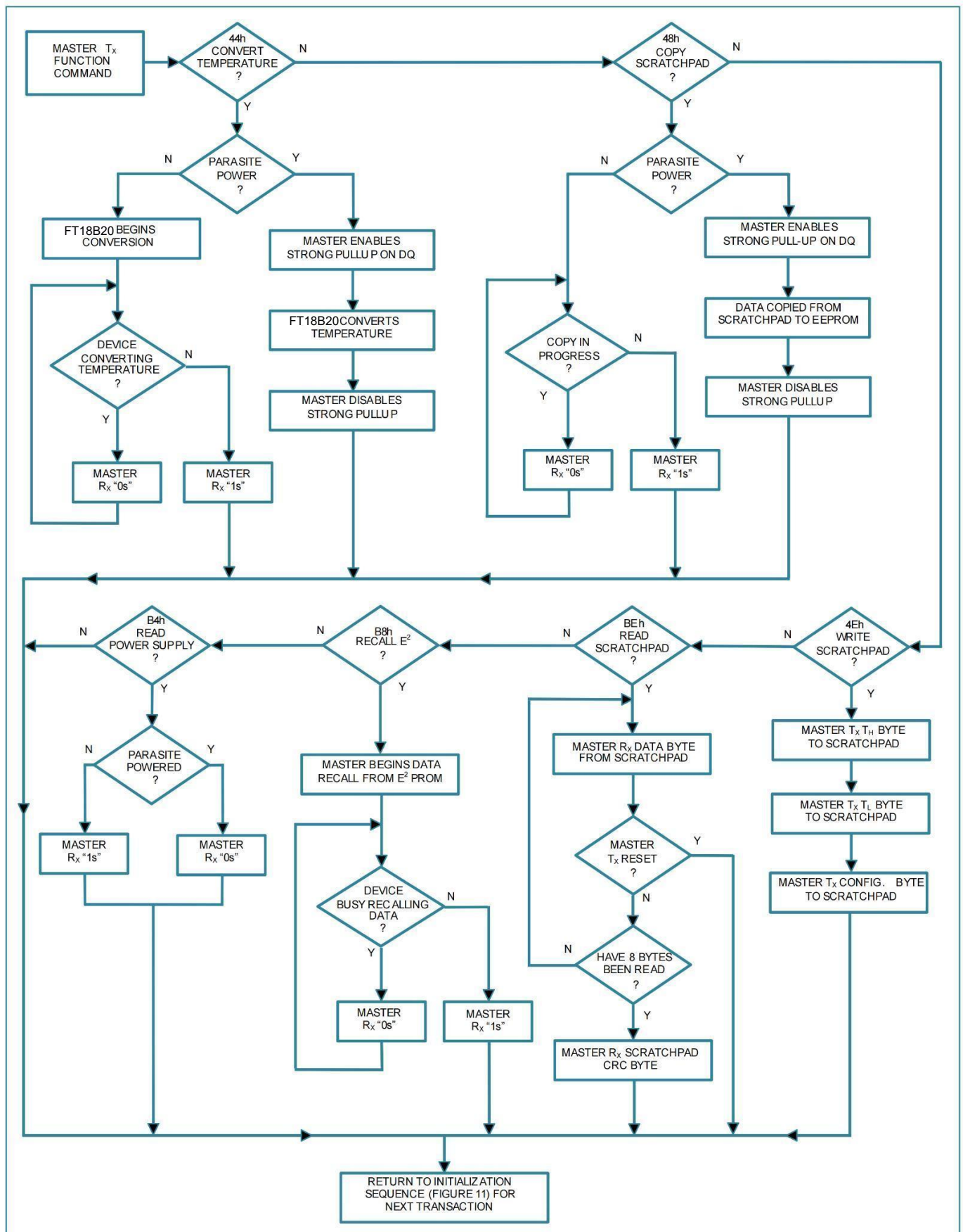
Figure 12. FT18B20 function instruction flowchart
