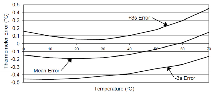
FT18B20 Typical Error Curve
