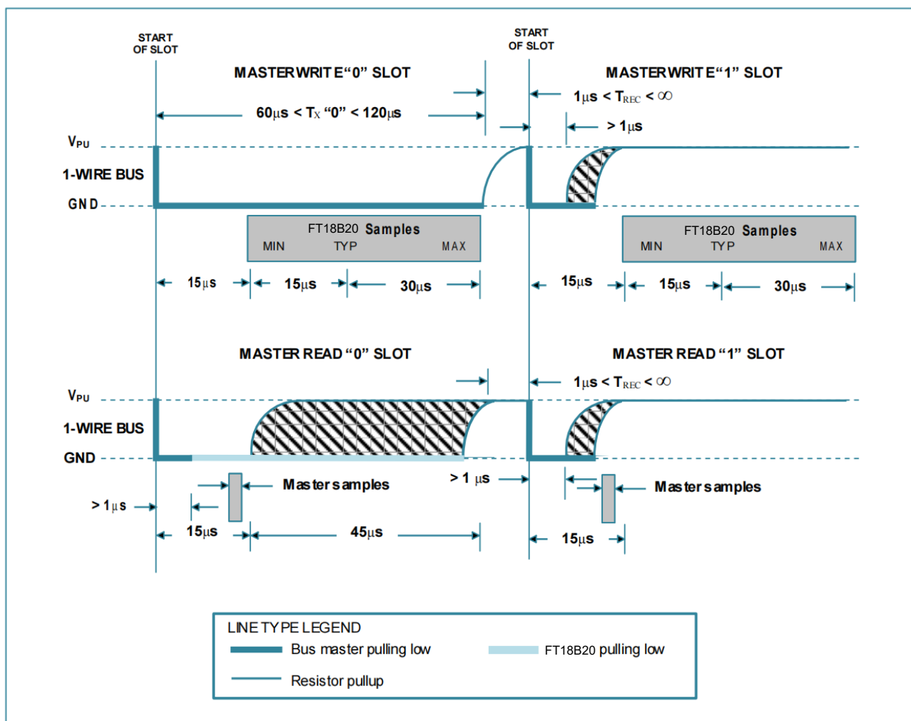
Figure 14. Read/Write Time Slot Timing Diagram
