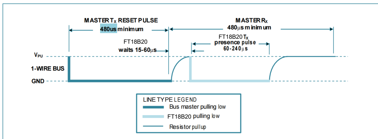
Figure 13. Initialization Timing
