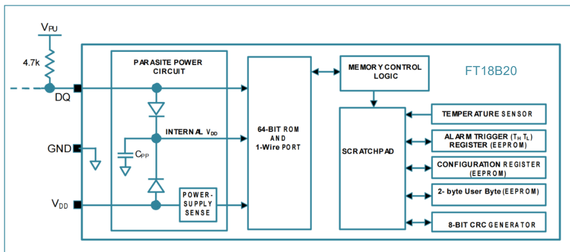
Figure 1. FT18B20 Block Diagram
