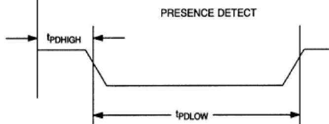
Figure 18. Timing Diagrams
