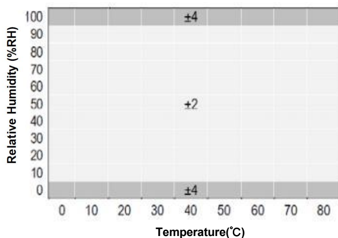
Figure 4 Tolerance of FHT31 under total temperature conditions
