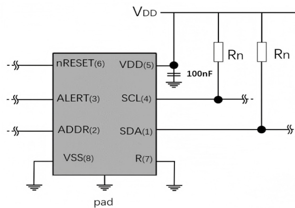
Figure 6. Typical Application Circuit.
