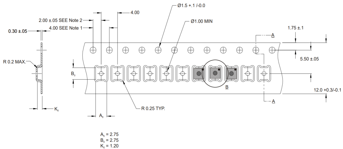
Figure 10. Dimensions of tape for chip transport.
