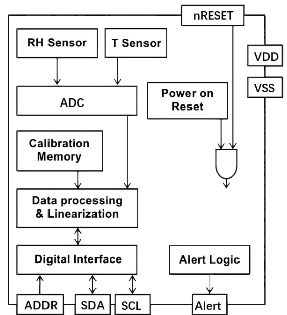
Figure 2. Functional block diagram of FHT31
