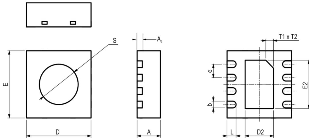
Figure 8. Dimensional drawing of FHT31 sensor package.
