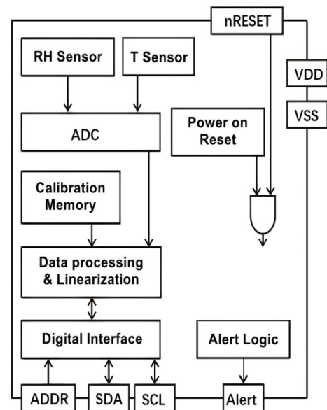
Figure 2. Functional block diagram of SHT30-P-NF
