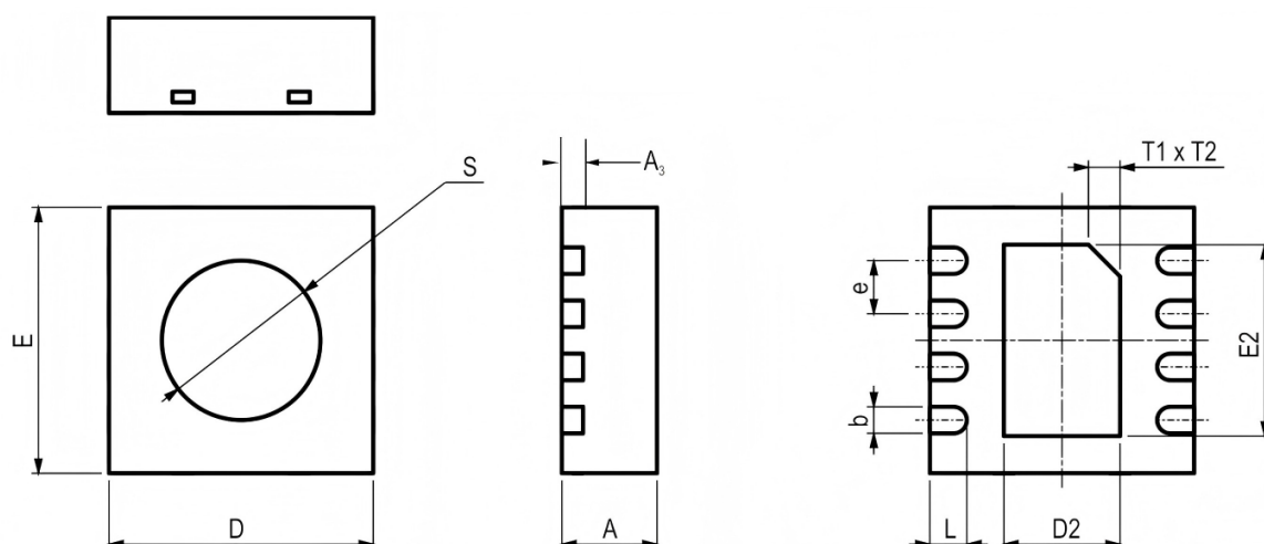
Figure 7 . Dimensional drawing of SHT30-P-NF sensor package.
