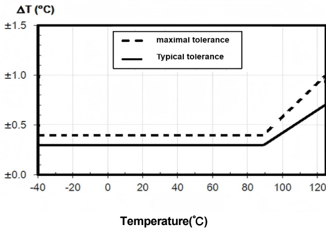
Figure 4 . Temperature accuracy of SHT30-P-NF
