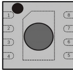
DFN-8 TOP VIEW
