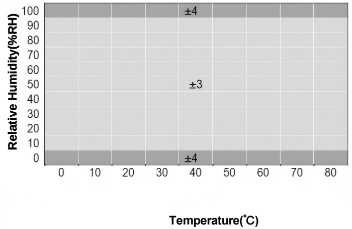
Figure 3.1 Tolerance of SHT30-P-NF under different temperature conditions
