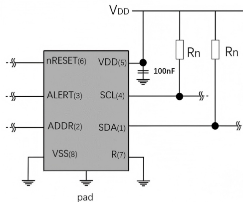
Figure 5. Typical Application Circuit.
