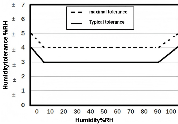
Figure 3 . Tolerance of RH at 25°C for SHT30-P-NF
