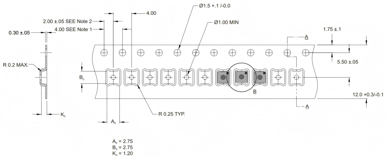
Figure 9. Dimensions of tape for chip transport.
