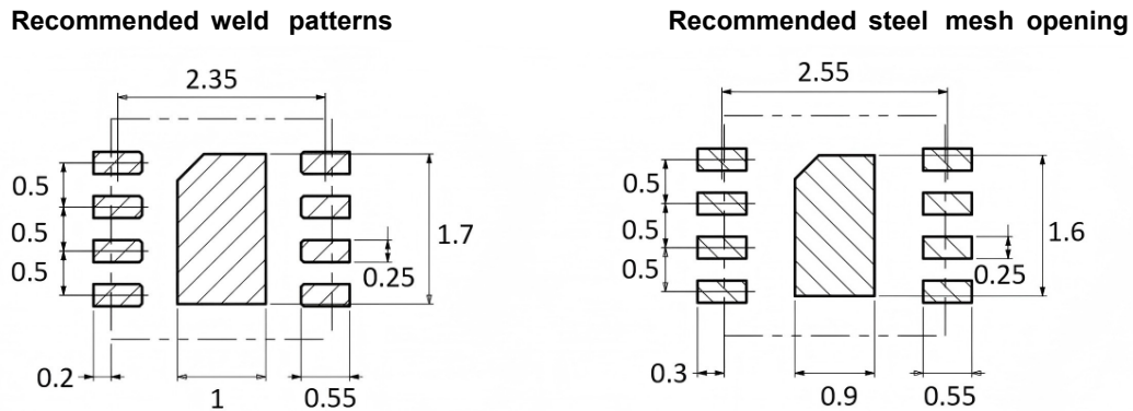
Figure 8. Recommended metal land pattern and stencil apertures for the SHT30-P-NF.
