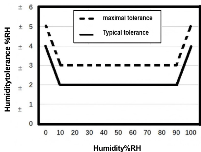
Figure 3. Tolerance of RH at 25°C for SHT31-P-NF
