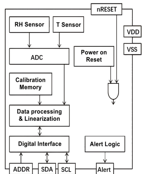
Figure 2 . Functional block diagram of SHT31-P-NF
