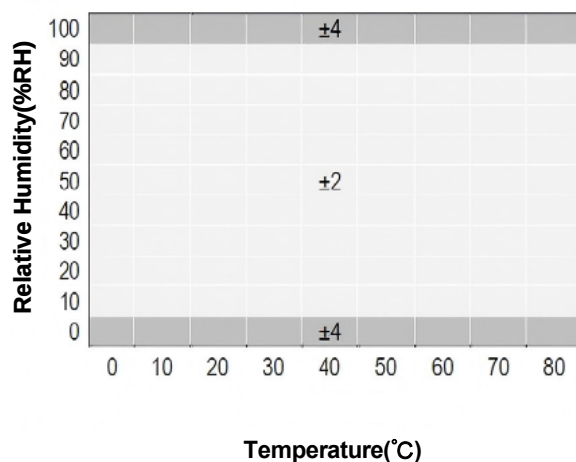
Figure 4 Tolerance of SHT31-P-NF under total temperature conditions
