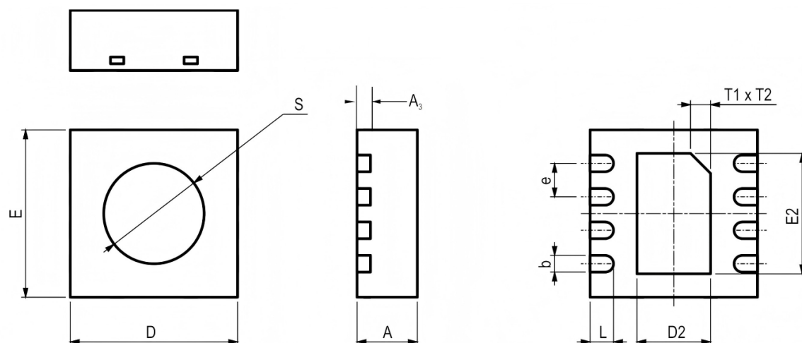
Figure 8. Dimensional drawing of SHT31-P-NF sensor package.
