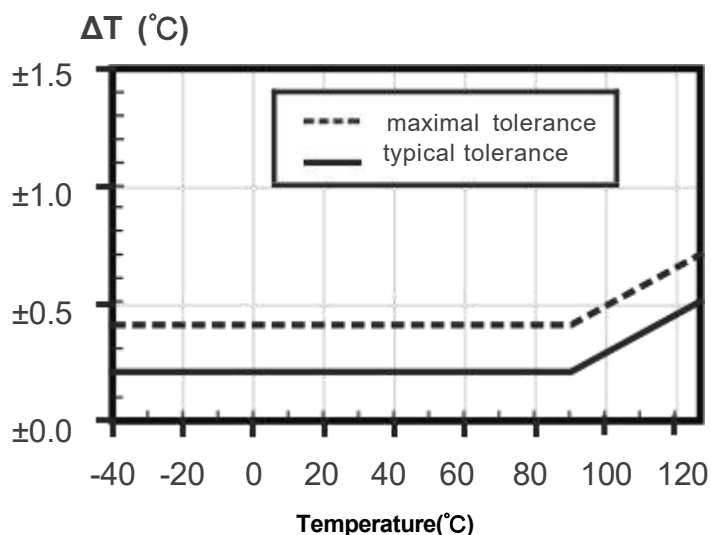
Figure 5. Temperature accuracy of SHT31-P-NF
