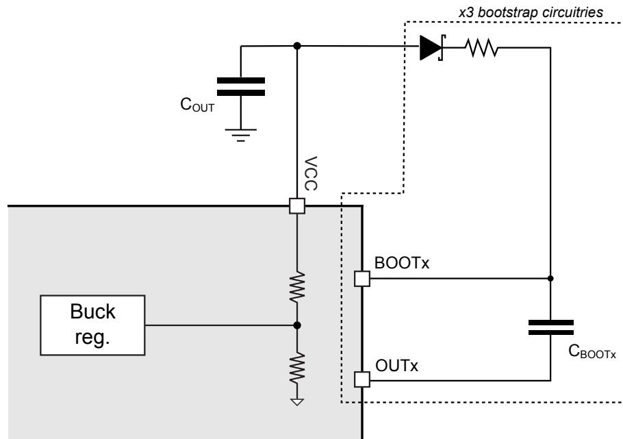
Figure 19. External bootstrap diode configuration
