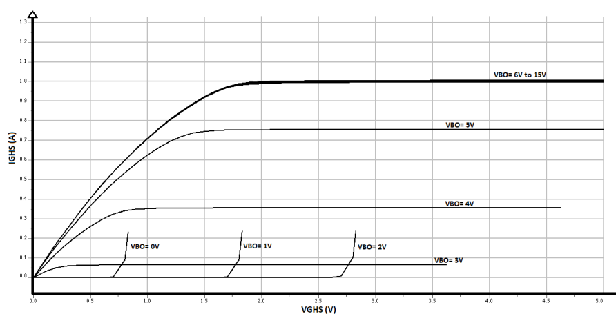
Figure 17. High-side gate driver output characteristic in UVLO range
