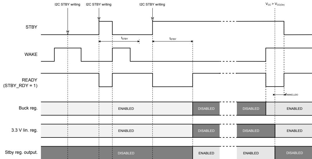
Figure 23. Standby timings
