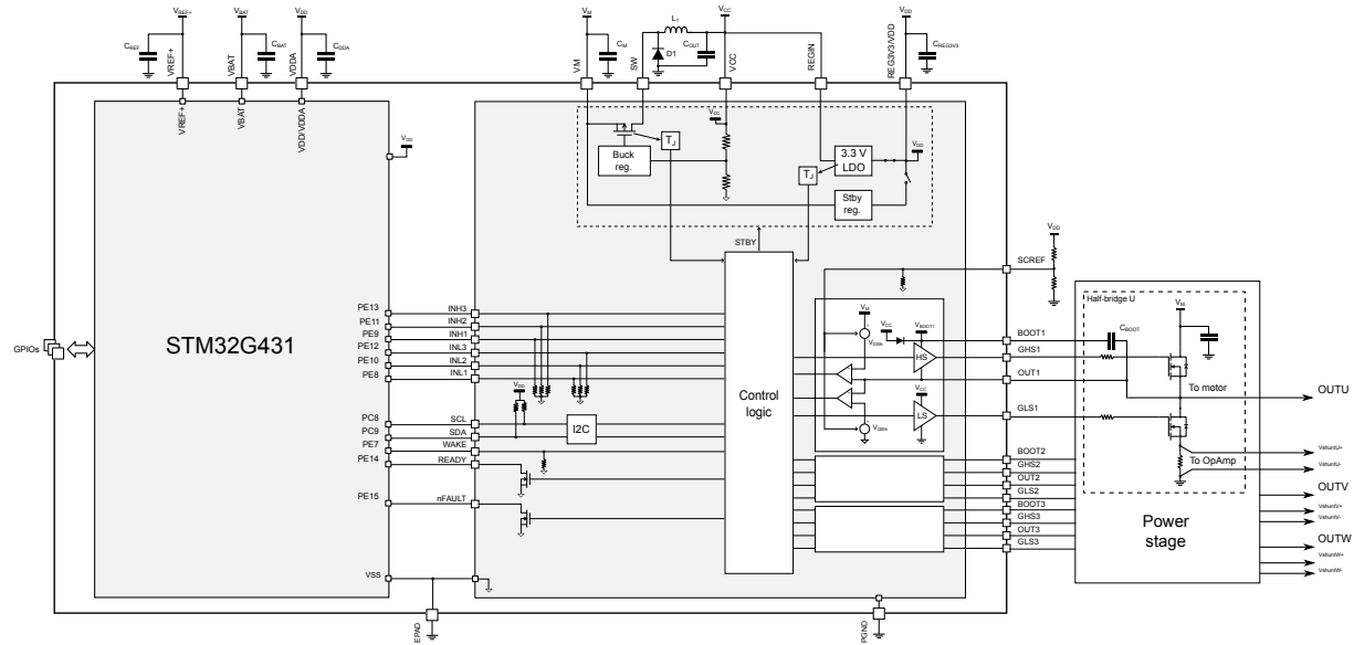
Figure 1. STSPIN32G4 system-in-package block diagram
