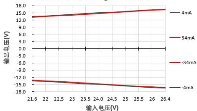
输出电压Vs输入电压@A2415LS-1WN
