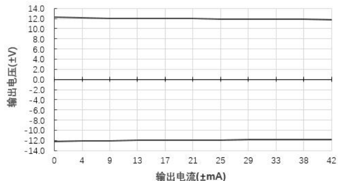
输出电压Vs输出电流(Vin=12V)@A1212LS-1WN
