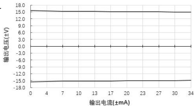
输出电压Vs输出电流(Vin=12V)@A1212LS-1WN
