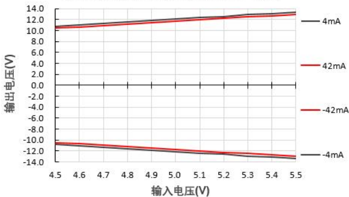
输出电压Vs输入电压@A0512LS-1WN
