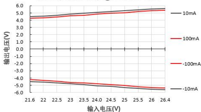
输出电压Vs输入电压@A2405LS-1WN
