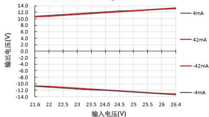
输出电压Vs输入电压@A2412LS-1WN
