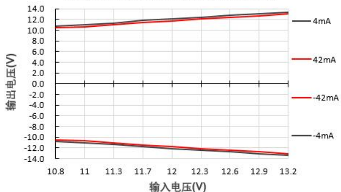
输出电压Vs输入电压@A1212LS-1WN
