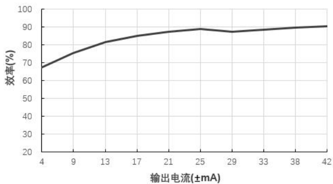
效率Vs输出电流(Vin=24V)@A2412LS-1WN
