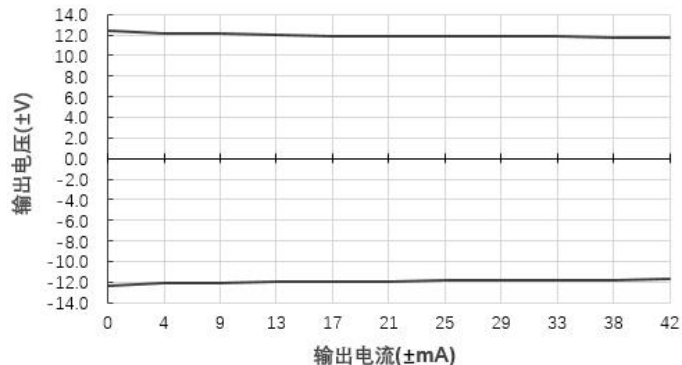
输出电压Vs输出电流(Vin=5V)@A0512LS-1WN
