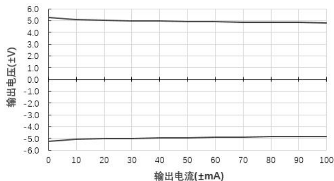
输出电压Vs输出电流(Vin=24V)@A2405LS-1WN
