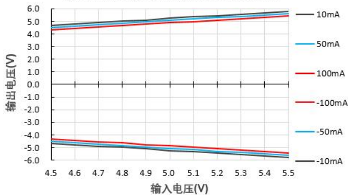
输出电压Vs输入电压@A0505LS-1WN
