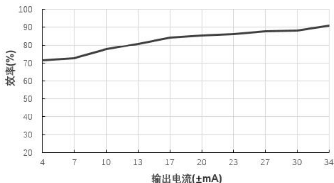
效率Vs输出电流(Vin=24V)@A2415LS-1WN
