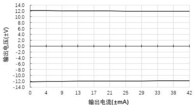
输出电压Vs输出电流(Vin=24V)@A2412LS-1WN
