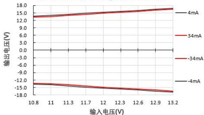
输出电压Vs输入电压@A1215LS-1WN
