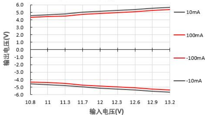
输出电压Vs输入电压@A1205LS-1WN
