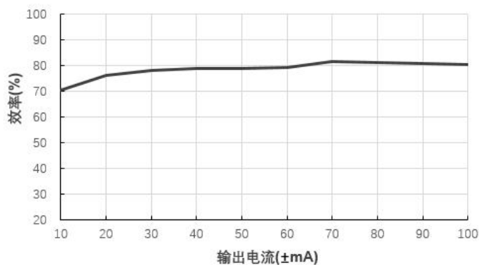
效率Vs输出电流(Vin=24V)@A2405LS-1WN
