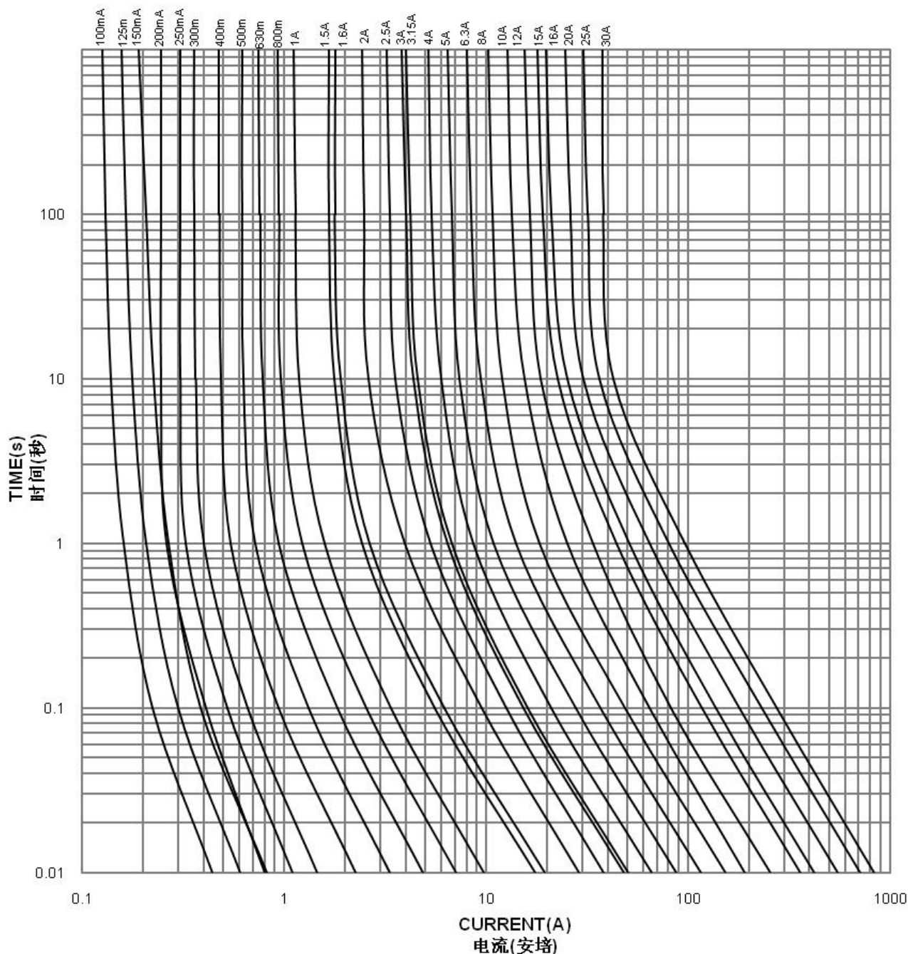
61NM RoHS Average I-T Characteristics Curve(For Reference Only) 61NM RoHS 平均I-T曲线图(供参考)
