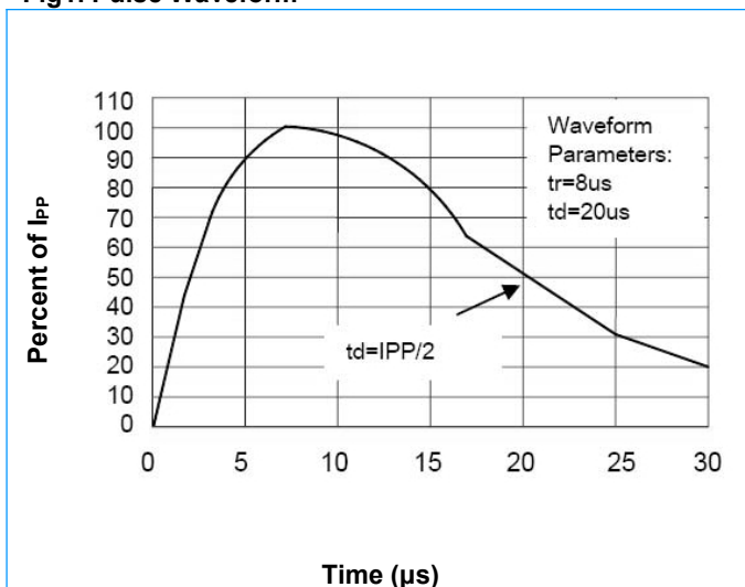
Fig1. Pulse Waveform
