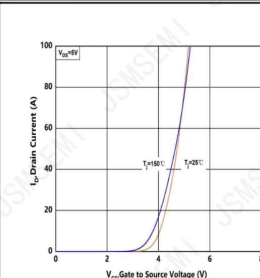
Figure.2 Transfer Characteristic for Various Junction Temperatures
