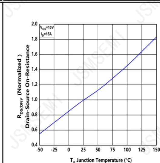
Figure.4 Typical On-Resistance vs Junction Temperature
