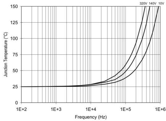
Figure 35. XL2110S/XL2113S TJ vs. Frequency (IRFPE50) R_{GATE} = 10\Omega , V_{CC} = 15V
