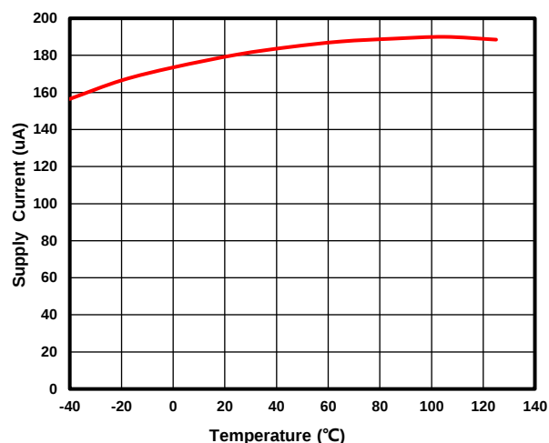
Figure 2. Supply Current vs. Temperature
