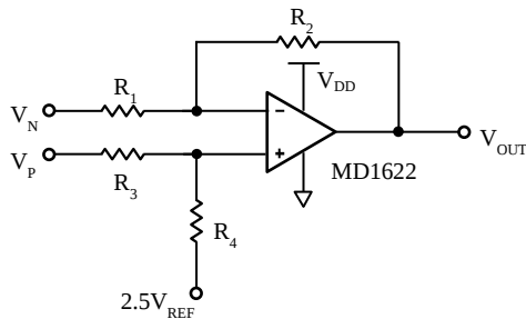
Figure 25. Differential Amplifier
