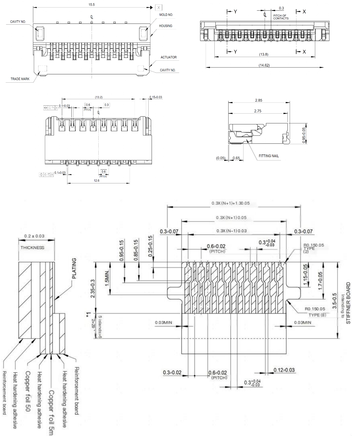
Figure 14 Connector size and FPC layout recommended size
