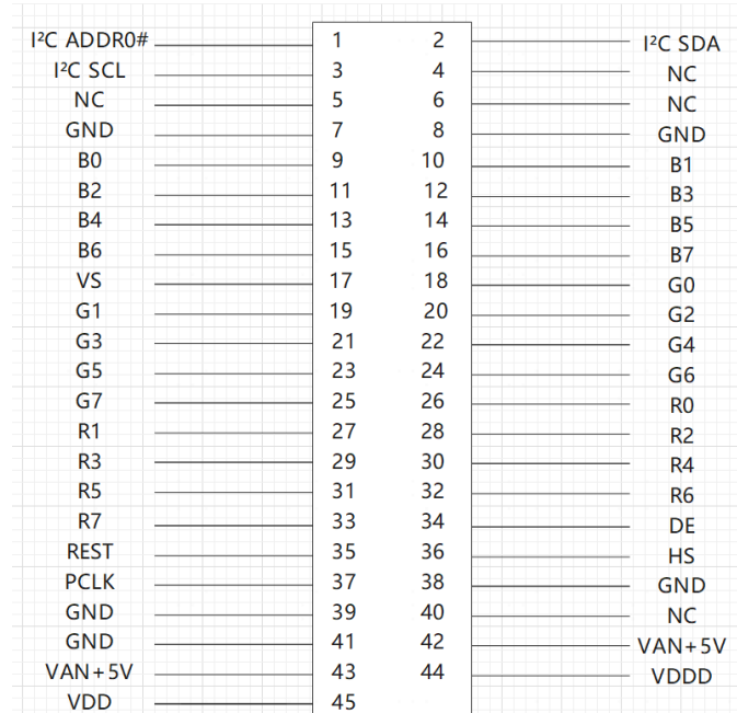
Figure 2 Schematic symbols for the micro display interface
