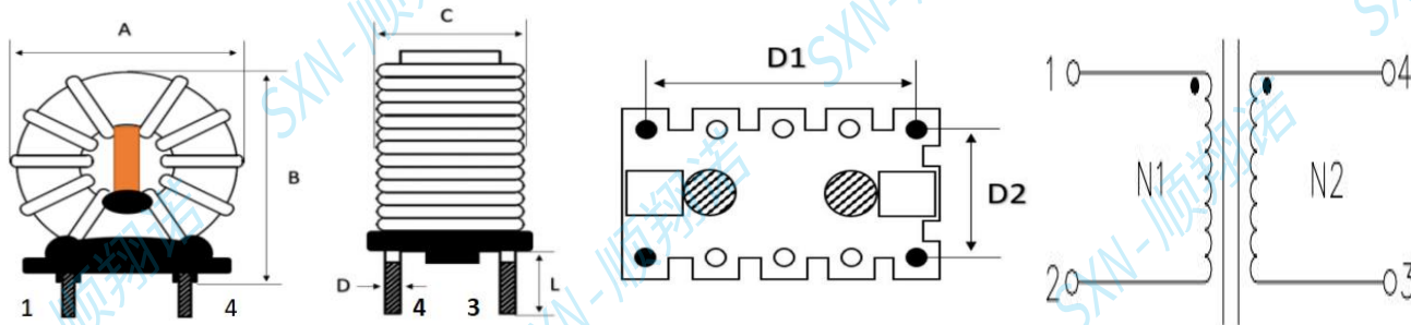
SCHEMATIC
