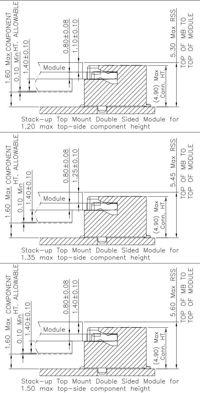
Assembly stack height schematic diagram
