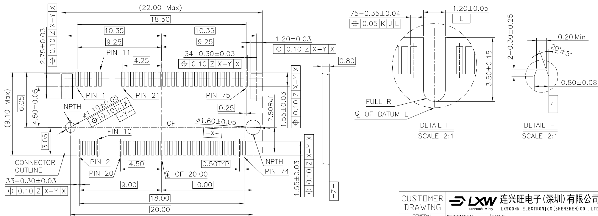
RECOMMENDED PCB LAYOUT(TOP VIEW) DEFAULT TOLERANCE \pm 0.05\text{MM}
