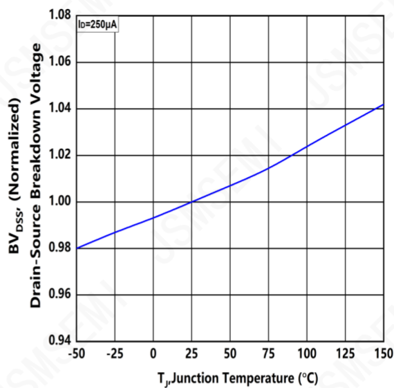
Figure.6 Typical Breakdown Voltage vs Junction Temperature
