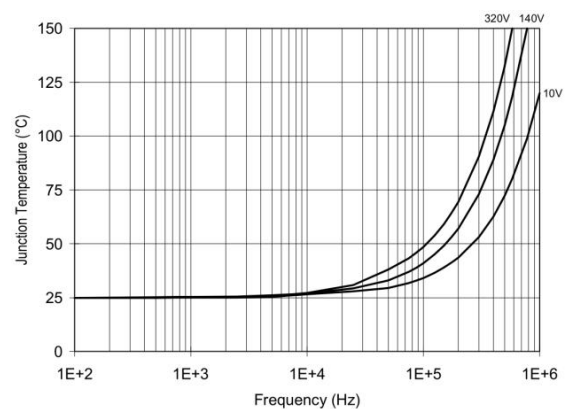
Figure 34. XL2110S/XL2113S TJ vs. Frequency (IRFBC40) RGATE = 15Ω, VCC = 15V
