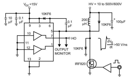
Figure 2. Floating Supply Voltage Transient Test Circuit
