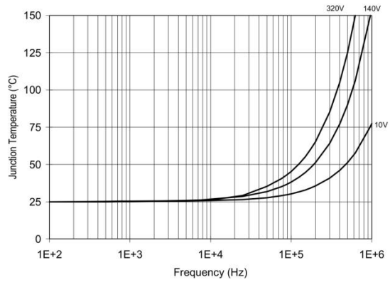
Figure 32. XL2110S/XL2113S TJ vs. Frequency (IRFBC20) RGATE = 33Ω, VCC = 15V
