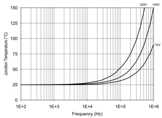
Figure 30. XL2110/XL2113 TJ vs. Frequency (IRFBC40) RGATE = 15Ω, VCC = 15V
