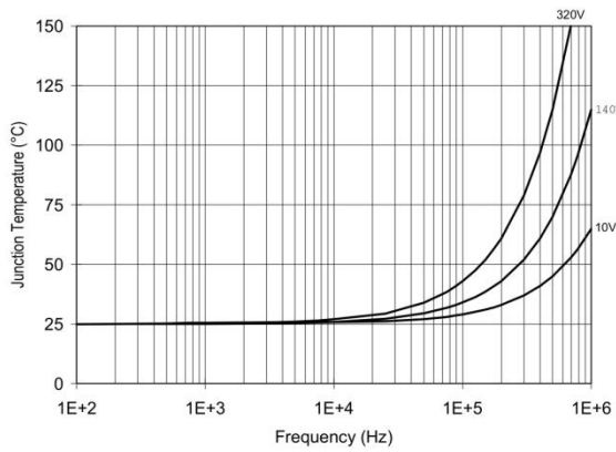
Figure 29. XL2110/XL2113 TJ vs. Frequency (IRFBC30) RGATE = 22Ω, VCC = 15V
