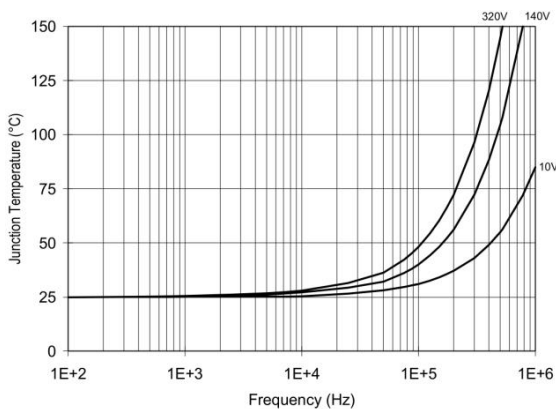
Figure 33. XL2110S/XL2113S TJ vs. Frequency (IRFBC30) RGATE = 22Ω, VCC = 15V
